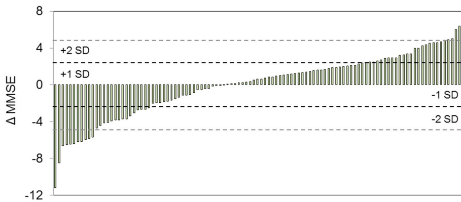
Fig. 4. Distribution of individual discrepancies between the clinical and calculated cognitive performance. The discrepancy in mini mental status examination (MMSE) values ( \Delta\text{MMSE} ) is illustrated by a waterfall plot representing the proposed surrogate score for individual cognitive reserve. \pm 1 standard deviation (SD) illustrated by black dashed line, and \pm 2 SD illustrated by grey dashed line are provided as previously published for MMSE test-retest studies.
