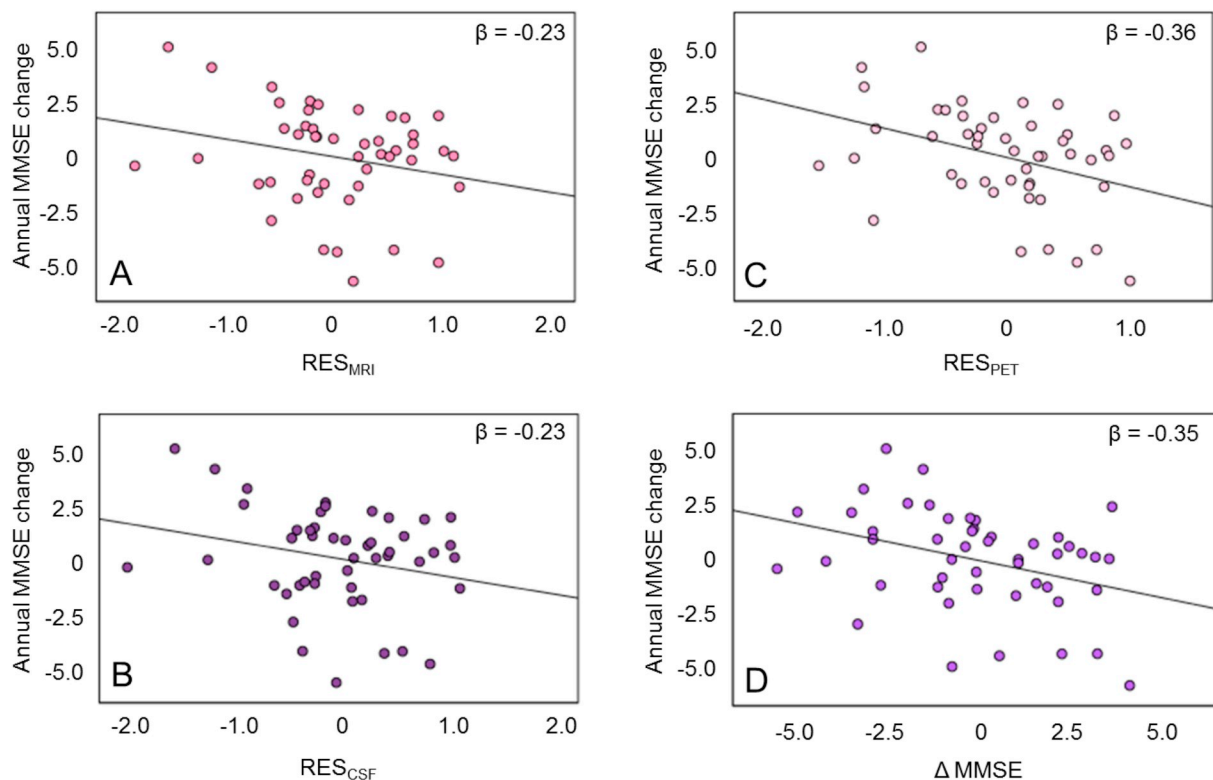
Fig. 5. Correlation between change in MMSE scores to clinical follow-up and biomarker findings. Presented are the correlations of stand-alone regressions residuals ( \text{RES}_{\text{MRI}} , \text{RES}_{\text{CSF}} , \text{RES}_{\text{PET}} ) of magnetic resonance imaging (MRI; A), total-tau in cerebrospinal fluid (CSF; B) and FDG positron emission tomography (PET; C) as well as the surrogate score of cognitive reserve ( \Delta\text{MMSE} ; D) with the annual MMSE change during clinical follow-up. Values are presented as residuals (res.) from the regression analysis.
