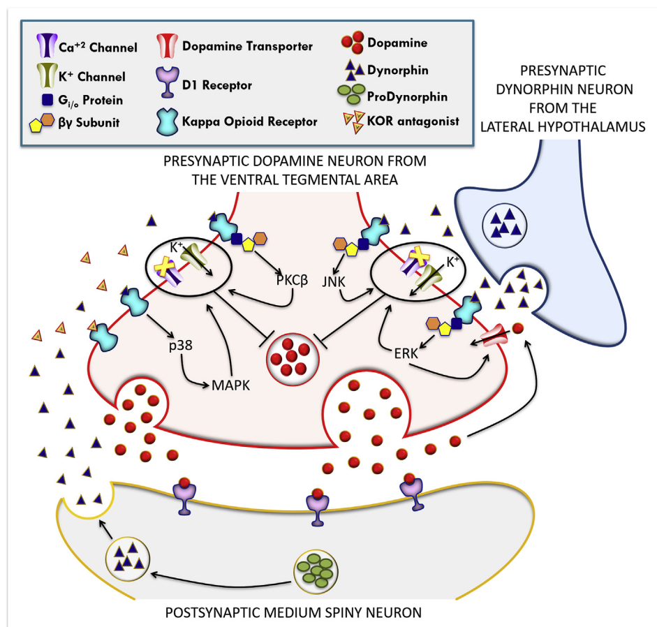
Fig. 2. Schematic of mechanisms through which kappa opioid receptors regulate dopamine release in the nucleus accumbens. Activation of kappa opioid receptors (KORs) on dopamine terminals results in inhibition of dopamine release. This occurs via coupling of KORs with Gi/o proteins activating one or more kinases (PKC \beta , JNK, or ERK) and hyperpolarizing the cell via increasing K ^{+} conductance or inhibition of Ca ^{2+} channel function. Activation of KORs also increases p38 expression resulting in the activation of MAPK and further hyperpolarization of the cell. Activation of KORs has also been shown to increase DAT function, accelerating uptake. Dynorphin, in the NAC, is released from D1R-containing medium spiny neurons and probably from afferents from the lateral hypothalamus. KOR, kappa opioid receptor; D1R, dopamine type 1 receptor; DAT, dopamine transporter; Ca ^{2+} , calcium; K ^{+} , potassium; MAPK, mitogen-activated protein kinases; JNK, c-Jun N-terminal kinases; pDYN, prodynorphin; cAMP, cyclic adenosine monophosphate; CREB, cAMP response element-binding protein; BDNF, brain derived neurotrophic factor; AC, adenylyl cyclase; PKC, protein kinase C.
