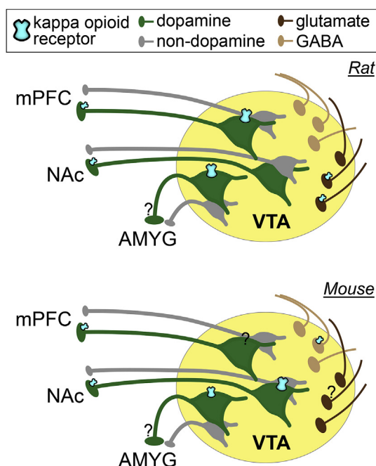
Fig. 1. Functional kappa opioid receptors are expressed on specific VTA circuit elements. In rat (top), dopamine cell bodies in the VTA that project to the medial prefrontal cortex (mPFC) and the amygdala (AMYG) are inhibited by kappa opioid receptor (KOR) activation, which open G protein coupled inwardly rectifying K^+ channels. Dopamine neurons that project to the nucleus accumbens (NAc) do not show this response, however KOR activation inhibits release at dopamine terminals in the NAc. Excitatory glutamatergic inputs onto VTA neurons are also inhibited by KOR activation. These effects may also depend upon the source of the afferents and the projection target of the post-synaptic cell. In mouse (bottom), most NAc-projecting VTA dopamine cell bodies and some amygdala-projecting VTA dopamine neurons are directly inhibited by KOR activation. It is unknown if KOR activation also inhibits mPFC-projecting VTA dopamine neurons in mice. KORs also inhibit GABA release onto VTA neurons in mice.
