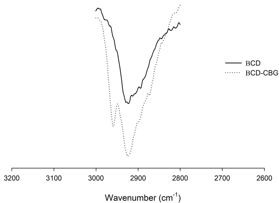
Fig. 4. FTIR spectra of \beta -CD and \beta -CD+CBG inclusion complexes obtained in the spectral range of 3200–2600 \text{cm}^{-1} .
