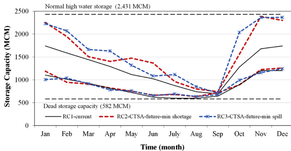
Fig. 11. Optimal future rule curves of Ubolrat Reservoir using minimize water shortage and minimize excess spill water with CTSA model.
