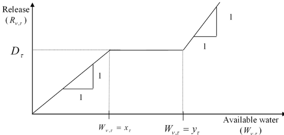
Fig. 1. Standard operating rule.
