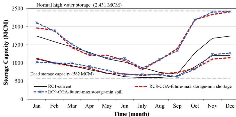
Fig. 14. Optimal future rule curves of Ubolrat Reservoir using maximize stored water at end of wet season with CGA model.
