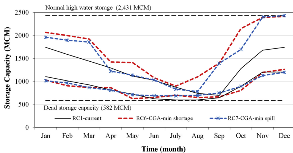
Fig. 9. Optimal historic rule curves of Ubolrat Reservoir using minimize water shortage and minimize excess spill water with CGA model.
