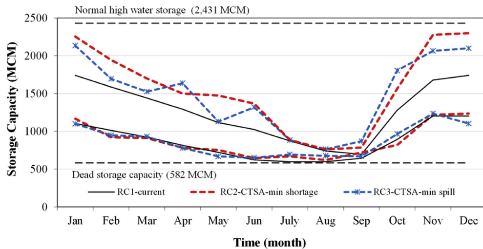
Fig. 7. Optimal historic rule curves of Ubolrat Reservoir using minimize water shortage and minimize excess spill water with CTSA model.
