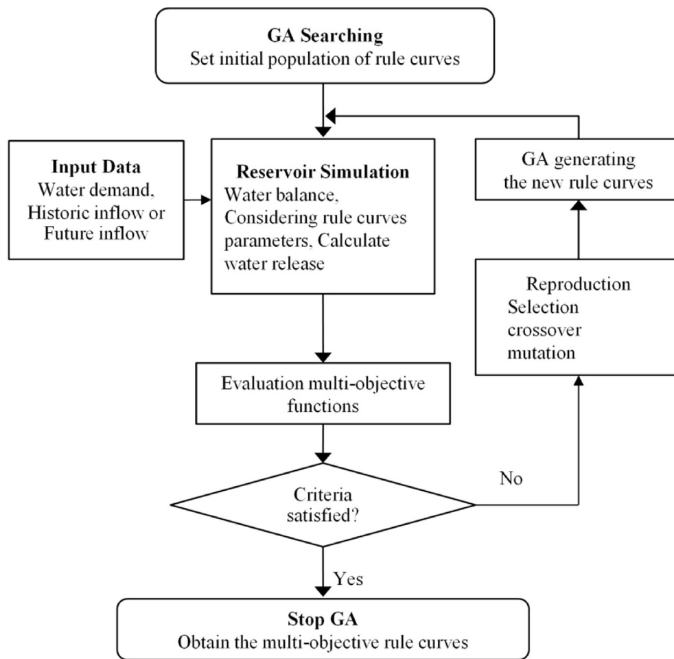
Fig. 3. Conditional genetic algorithm connecting reservoir simulation for searching rule curves.
