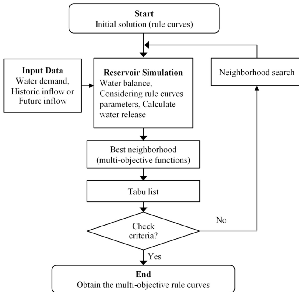
Fig. 2. Conditional tabu search algorithm connecting reservoir simulation for searching rule curves.
