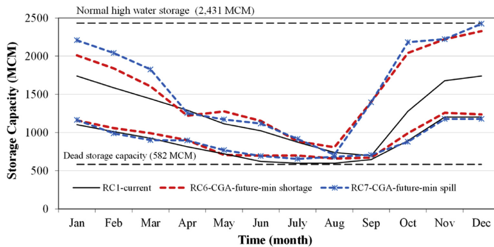
Fig. 13. Optimal future rule curves of Ubolrat Reservoir using minimize water shortage and minimize excess spill water with CGA model.
