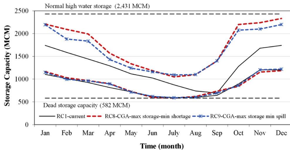
Fig. 10. Optimal historic rule curves of Ubolrat Reservoir using maximize stored water at end of wet season with CGA model.
