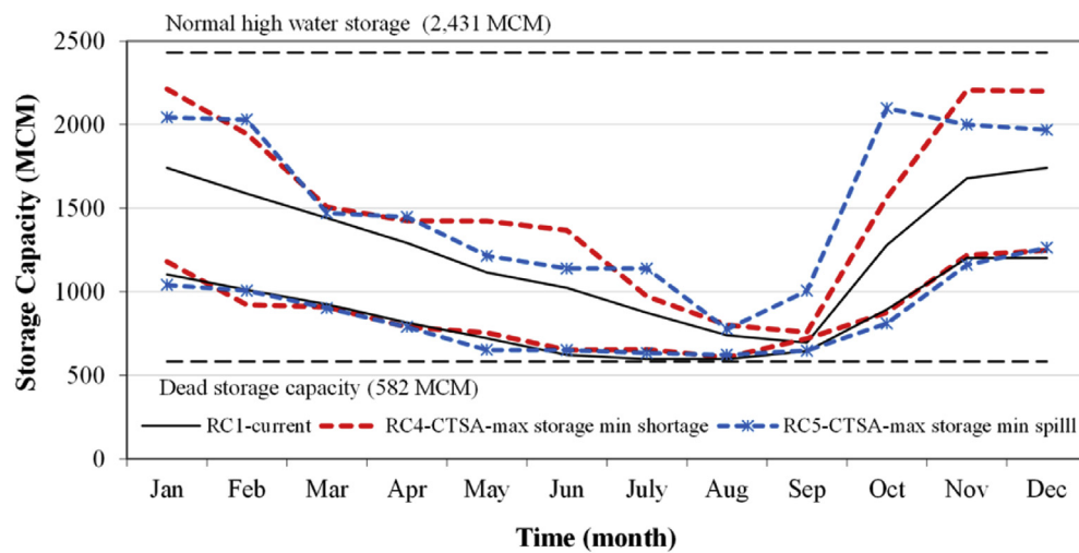
Fig. 8. Optimal historic rule curves of Ubolrat Reservoir using maximize stored water at end of wet season with CTSA model.
