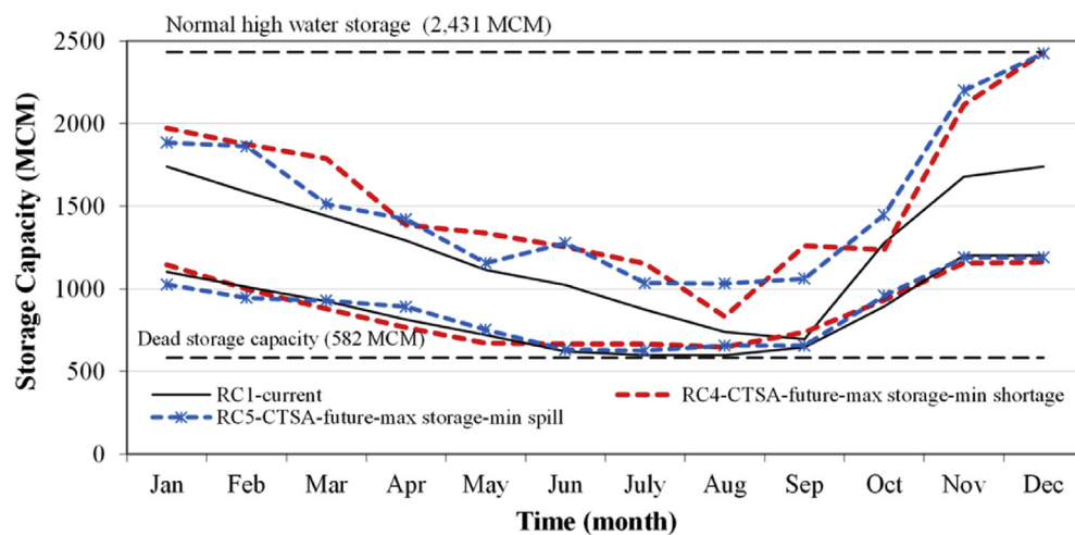
Fig. 12. Optimal future rule curves of Ubolrat Reservoir using maximize stored water at end of wet season with CTSA model.
