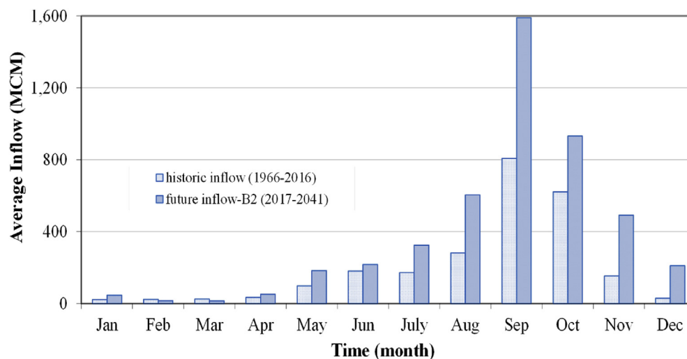
Fig. 6. Historic inflow and future inflow of Ubolrat Reservoir.
