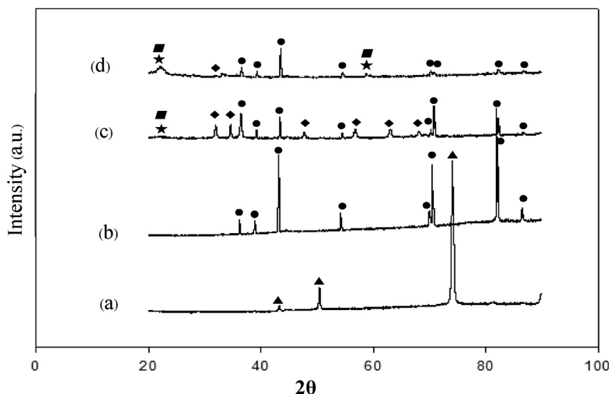
Fig. 1. XRD patterns of (a) Cu plate, (b) Zn deposited at a current density of 0.1 \text{ A/cm}^2 with 1 \text{ M ZnSO}_4 (fresh electrode), (c) Zn deposited at a current density of 0.1 \text{ A/cm}^2 with 1 \text{ M ZnSO}_4 after the performance test and (d) Zn deposited at a current density of 0.1 \text{ A/cm}^2 with 0.5 \text{ M ZnSO}_4 after the performance test.
