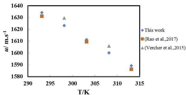
Fig. 5. Speed of sound ( u ) of IL against temperature ranges T = (293.15, 298.15, 303.15, 308.15 \text{ and } 313.15)\text{ K} compared to the literature values.
