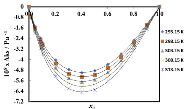
Fig. 11. Deviation in isentropic compressibility \Delta k_s , of the binary mixtures of \{[\text{C}_2\text{mim}][\text{BF}_4] (x_1) + \text{ethyl acetoacetate} (x_2)\} expressed in mole fraction of [\text{C}_2\text{mim}][\text{BF}_4] at T = (293.15, 298.15, 303.15, 308.15 \text{ and } 313.15) \text{ K} . The plot was fitted by using the Redlich-Kister equation.
