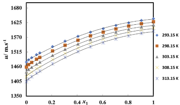
Fig. 6. Speed of sound ( u ) graph for the binary mixtures of \{[\text{C}_2\text{mim}][\text{BF}_4] (x_1) + \text{benzaldehyde} (x_2)\} at T = (293.15, 298.15, 303.15, 308.15 \text{ and } 313.15)\text{ K} .
