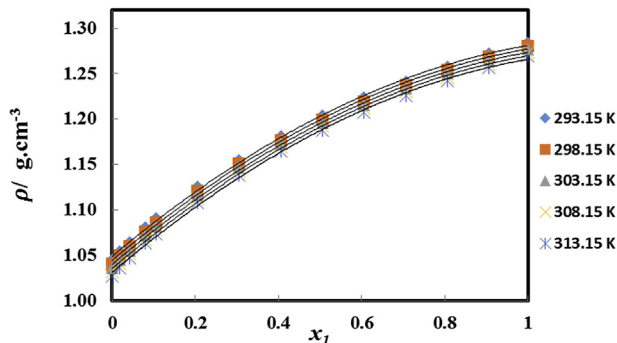
Fig. 3. Density of the binary mixtures of \{[\text{C}_2\text{mim}][\text{BF}_4] (x_1) + \text{benzaldehyde} (x_2)\} at T = (293.15, 298.15, 303.15, 308.15 \text{ and } 313.15)\text{ K} .
