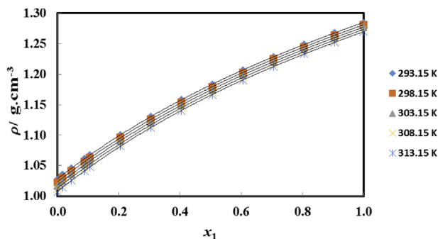
Fig. 4. Density of the binary mixtures of \{[\text{C}_2\text{mim}][\text{BF}_4] (x_1) + \text{ethyl acetate} (x_2)\} at T = (293.15, 298.15, 303.15, 308.15 \text{ and } 313.15)\text{ K} .
