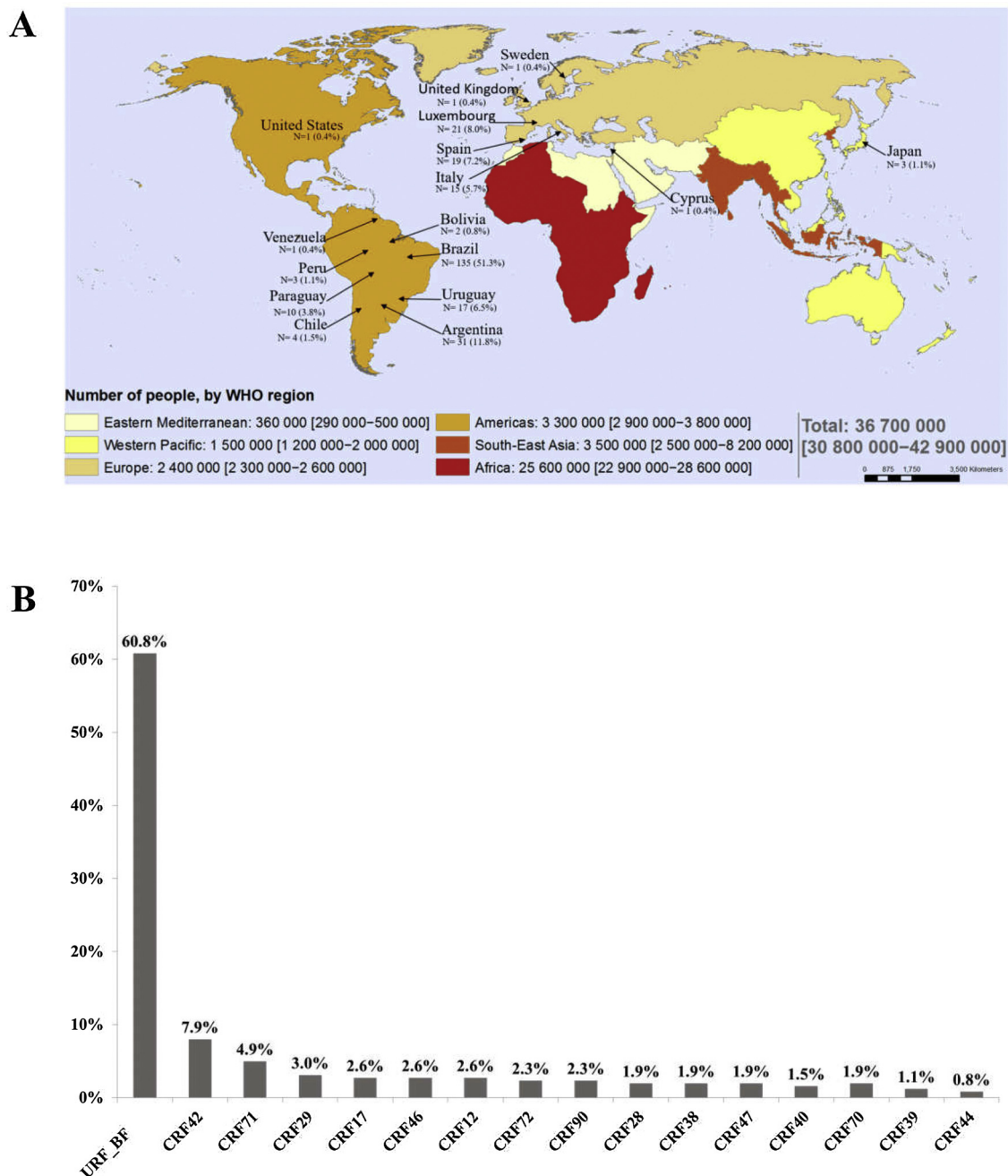
Fig. 1. Distribution of 265 HIV BF recombinant viruses (A) Geographic origin and worldwide distribution of the strains. (N) number of collected sequences in each country. The map shows the estimated number of people living with HIV in 2016 by WHO region. Figure adaptation from http://gamapserver.who.int/mapLibrary/Files/Maps/HIV_all_2016.png . (B) Genetic profile distribution among BF recombinant viruses circulating in the world. URF_BF: BF Unique Recombinant Forms. CRF: Circulating Recombinant Form.
