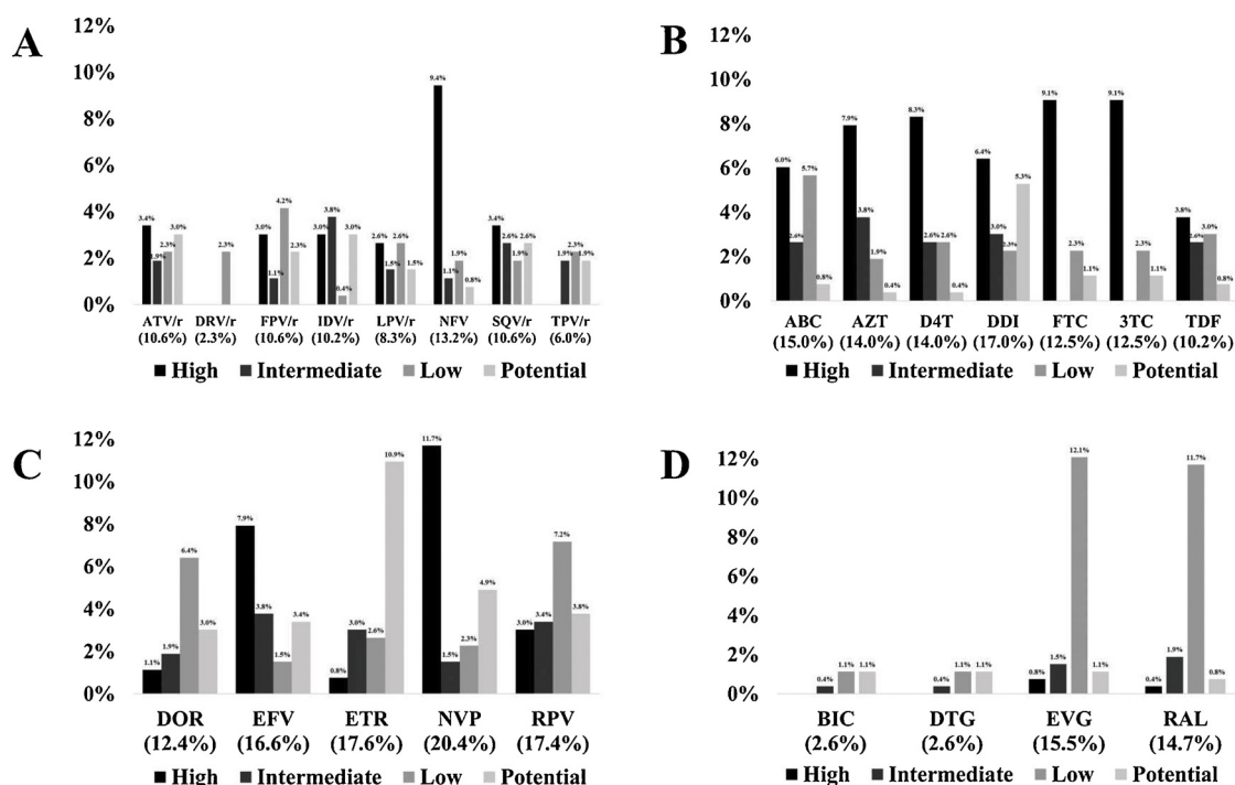
Fig. 6. Prevalence of antiretroviral resistance among HIV-1 BF recombinant sequences. Resistance to (A) Protease Inhibitors (PIs). (B) Nucleoside Reverse Transcriptase Inhibitor (NRTIs). (C) Non-Nucleoside Reverse Transcriptase Inhibitor (NNRTIs). (D) Integrase Strand Transfer Inhibitors (INSTIs). Protease Inhibitors: ATV (Atazanavir/ritonavir), DRV/r (Darunavir/ritonavir), FPV (Fosamprenavir/ritonavir), IDV/r (Indinavir/ritonavir), LPV/r (Lopinavir/ritonavir), NFV (Nelfinavir), SQV (Saquinavir/ritonavir) and TPV/r (Tipranavir/ritonavir). Nucleoside Reverse Transcriptase Inhibitors: ABC (Abavavir), AZT (Zidovudine), D4T (Stavudine), DDI (Didanosine), FTC (Emtricitabine), 3TC (Lamivudine) and TDF (Tenofovir). Non-Nucleoside Reverse Transcriptase Inhibitors: DOR (Doravirine), EFV (Efavirenz), ETR (Etravirine), NVP (Nevirapine) and RPV (Rilpivirin). Integrase Inhibitors: BIC (Bictegravir), DTG (Dolutegravir), EVG (Elvitegravir) and RAL (Raltegravir).
