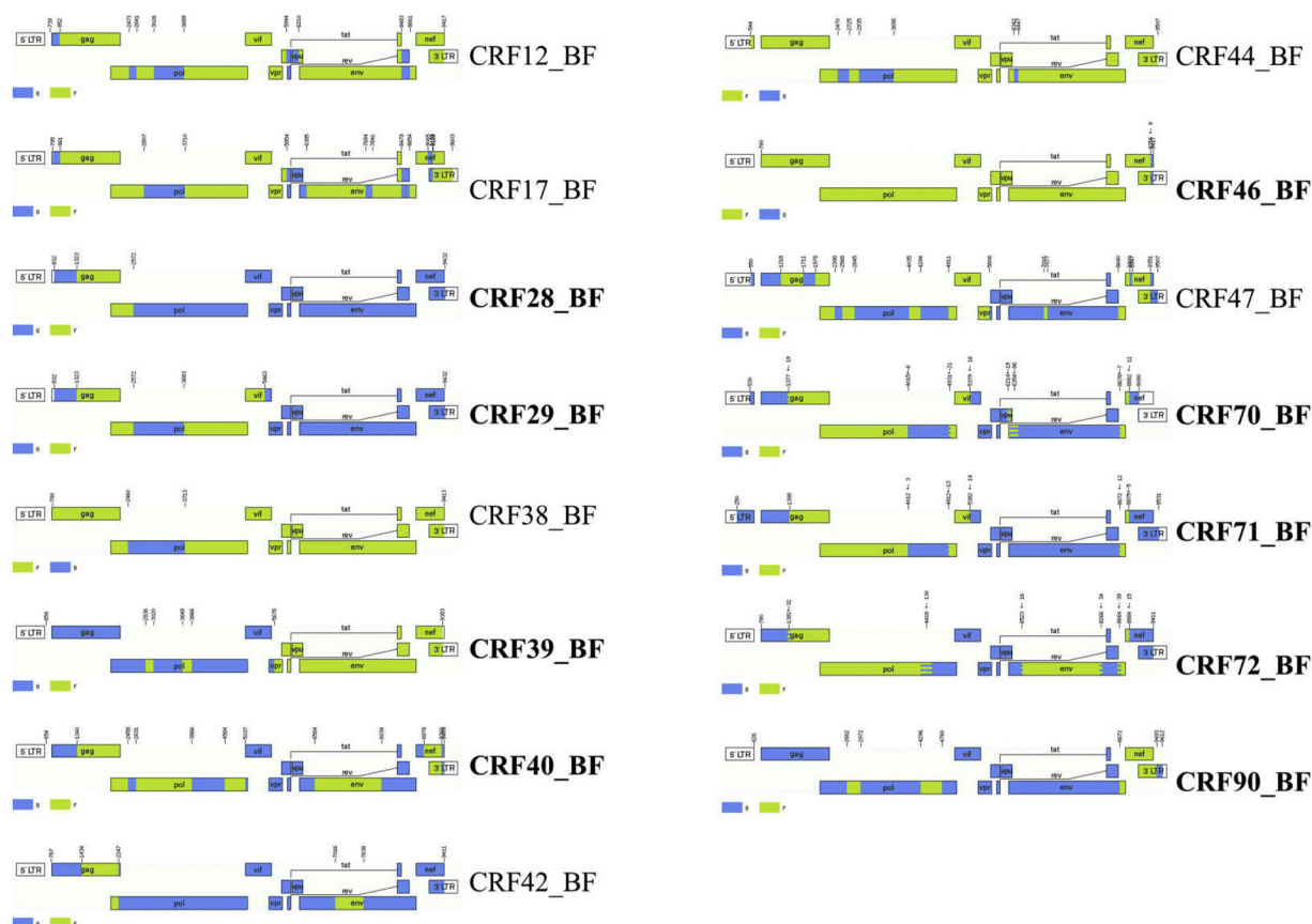
Fig. 2. Recombination patterns of the 15 CRF_BF circulating worldwide. The CRFs described in Brazil are identified in bold. Adapted from Los Alamos HIV sequence database ( https://www.hiv.lanl.gov/content/sequence/HIV/CRFs/CRFs.html ).
