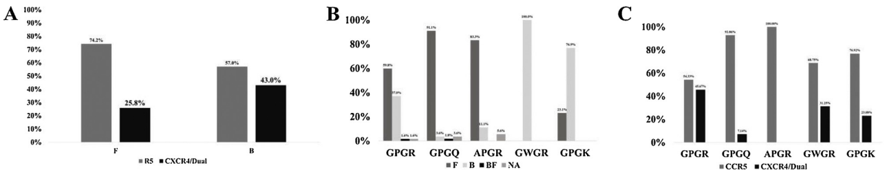
Fig. 5. Association between coreceptor usage, HIV-1 subtype and amino acid composition of the gp120 V3 region. (A) Frequency of R5 and X4/Dual tropic strains among subtypes B and F V3 sequences. (B) Classification of sequences with the most frequent motifs in the GP120 V3 loop according to the sequence subtype and (C) viral tropism.
