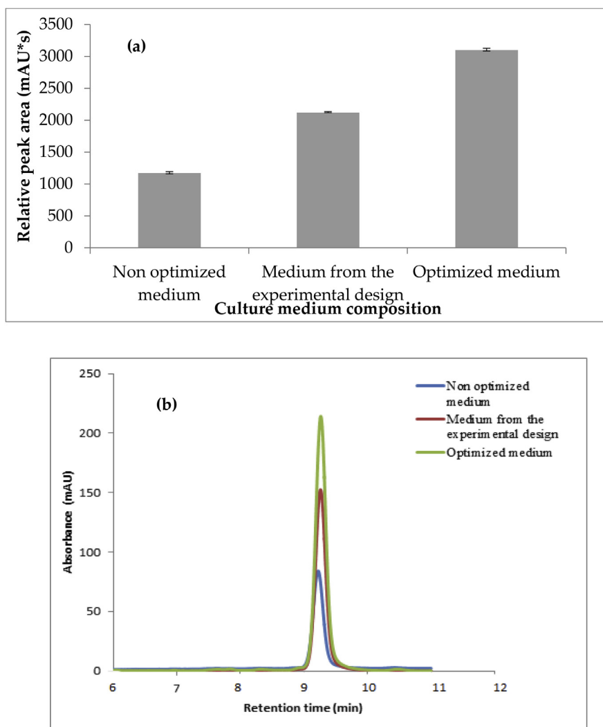
Fig. 13. (a) Relative peak areas of act-D eluted at t_R = 9.3 min in the chromatographic profile of the strain Streptomyces sp. GSBNT10, (b) Relative intensity of chromatographic peaks of act-D eluted t_R = 9.3 min by UV-DAD HPLC analysis (reversed phase C18 column, methanol-water 75:25, flow 1\text{ mLmin}^{-1} , detection at 440 nm).
