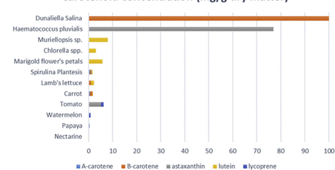
Fig. 2. Carotenoid content of different sources including flowers, vegetables and microalgae.
