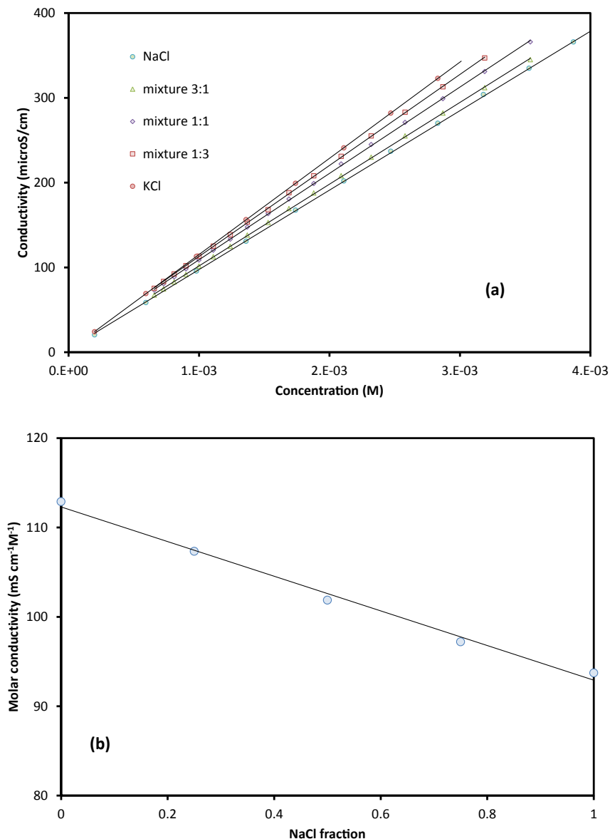
Fig. 2. (a) Conductivity of NaCl and KCl solutions. (b) Molar conductivity as the function of NaCl fraction (of NaCl-KCl mixtures).
