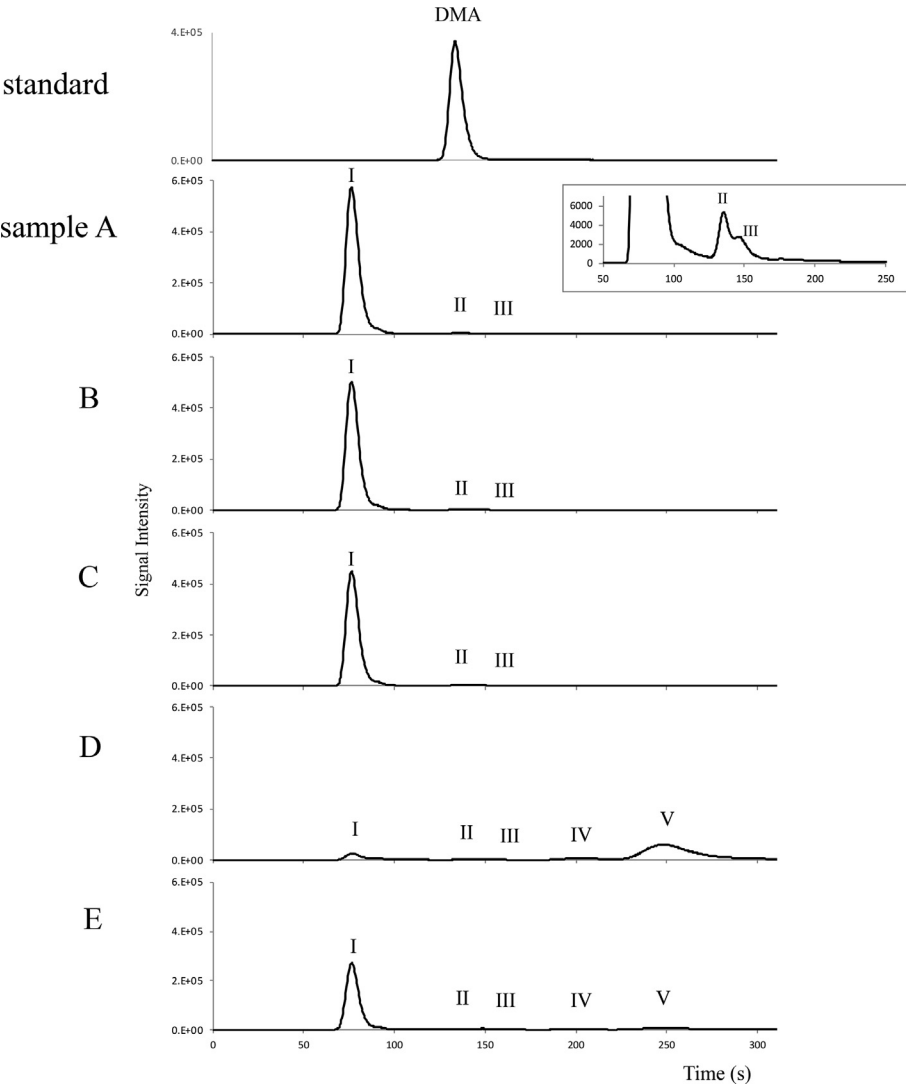
Fig. 2. Chemical conversion of AsSug328 treated with artificial gastrointestinal juice, enteric bacteria solution, and hydrogen peroxide solution, as determined by HPLC-ICP-MS. The arsenic compounds were separated by anion-exchange column chromatography on a PRP-X100 column. A: AsSug328 solution used in this study. B: Sample A treated with gastric juice for 4 h. C: Sample B treated with bile-pancreatic juice for 0.5 h. D: Sample C treated with enteric bacteria solution for 24 h. E: Sample D with hydrogen peroxide solution added.
