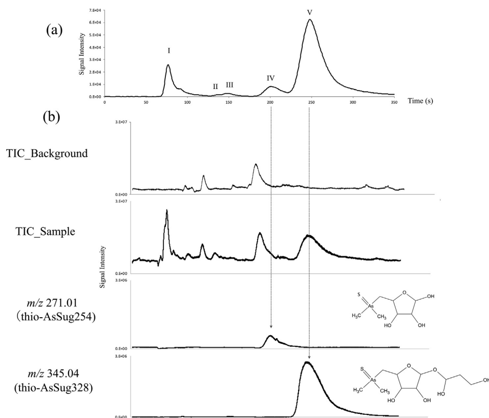
Fig. 3. Chemical conversion of AsSug328 treated in tandem with gastric juice, bile-pancreatic juice, and intestinal bacteria (sample D). Chromatograms of sample D as determined by (a) HPLC-ICP-MS and (b) HPLC-ESI-Q-TOF-MS using anion-exchange column chromatography on a PRP-X100 column. The background is for sample D, without AsSug328.
