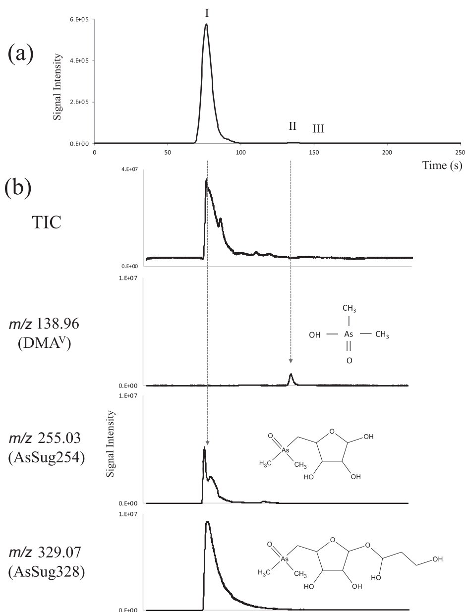
Fig. 1. (a) HPLC-ICP-MS and (b) HPLC-ESI-Q-TOF-MS chromatograms of AsSug328 used in this study (sample A). The arsenic compounds were separated by anion-exchange column chromatography on a PRP-X100 column.
