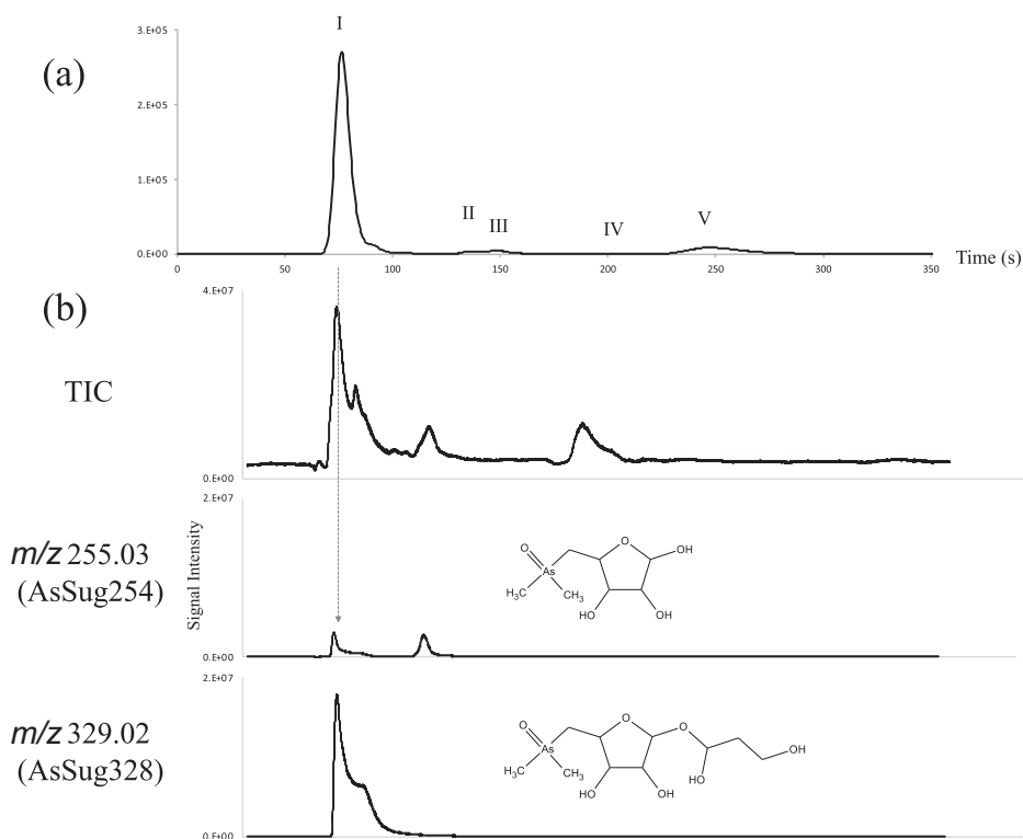
Fig. 4. Chromatogram of sample E after H_2O_2 was added to the enteric bacteria-treated sample, as determined by (a) HPLC-ICP-MS and (b) HPLC-ESI-Q-TOF-MS using anion-exchange column chromatography on a PRP-X100 column.
