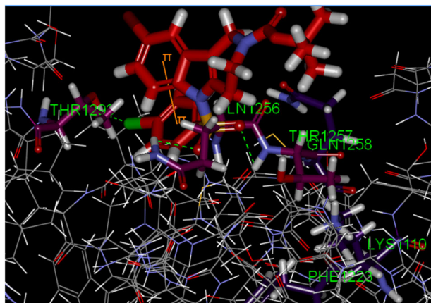
Fig. 6 Docking model of compounds 4c (red) with c-Met (3EFJ)
