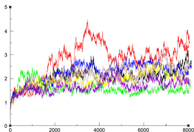
Fig. 8 Plot of RMSD for all the backbone atoms (Å) vs simulation time (ns) for 3EFJ in complex with compounds 4a–4g
