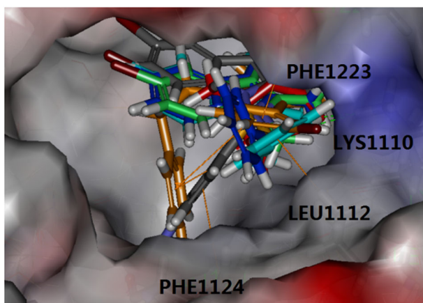
Fig. 5 Compact binding modes of all compounds (PDB:3EFJ)
