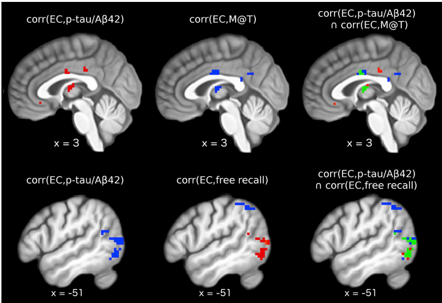
Fig. 2. Conjunction analysis. The main eigenvector centrality regression analysis was repeated twice, replacing p-tau/Aβ42 with score on memory alteration test (M@T) and score on delayed free recall of the free and cued selective reminding test, controlling for age, gender and level of education. Results were corrected for whole-brain multiple comparisons using identical methods to the main analysis. Top row left: significant positive correlations between EC and p-tau/Aβ42; top row middle: significant negative correlations between EC and M@T scores; top row right: green voxels display regions where EC correlated significantly with both p-tau/Aβ42 and M@T scores. Bottom row left: significant negative correlation between EC and p-tau/Aβ42; bottom row middle: significant positive (red) and significant negative (blue) correlations between EC and scores of delayed free recall; bottom row right: green voxels display regions where EC correlated significantly with both p-tau/Aβ42 and delayed free recall scores. (For interpretation of the references to color in this figure legend, the reader is referred to the web version of this article.)
