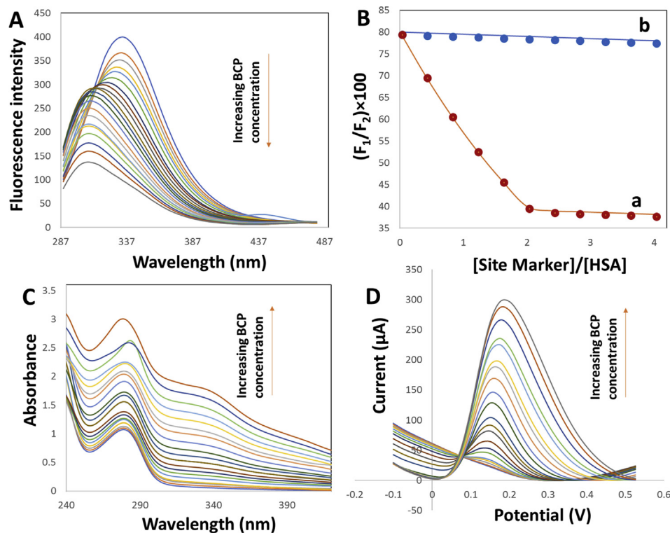
Fig. 4. (A) Fluorescence emission spectra of 2.0 \times 10^{-7} M HSA ( \lambda_{\text{ex}} = 280 nm) in the presence of increasing concentration of BCP ranging in 0 – 1.0 \times 10^{-6} M, (B) effects of Wr (curve a) and Ip (curve b) as site markers on the fluorescence of HSA-BCP, (C) UV-Vis absorption spectra of 1.0 \times 10^{-5} M HSA in the presence of increasing concentration of BCP ranging in 0 – 5.0 \times 10^{-5} M and (D) DPVs of 1.0 \times 10^{-5} M HSA in the presence of increasing concentration of BCP ranging in 0 – 5.0 \times 10^{-5} M.
