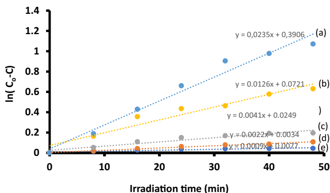
Fig. 10. First order kinetic plots for degradation methyl red: (a) 4.5 \times 10^{-5} , (b) 7.9 \times 10^{-5} , (c) 12.7 \times 10^{-5} , (d) 15.3 \times 10^{-5} and (e) 17.2 \times 10^{-5} using ClInOCPc/PAN as a catalyst. pH 7.4 buffer.
