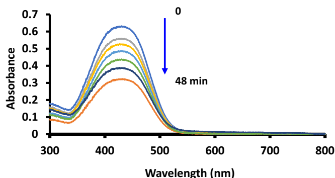
Fig. 9. Electronic absorption spectra changes 4.5 \times 10^{-5} \text{ mol/L} methyl red during visible light photocatalysis in the presence of ClInOCPc/PAN. pH 7.4 buffer employed.
