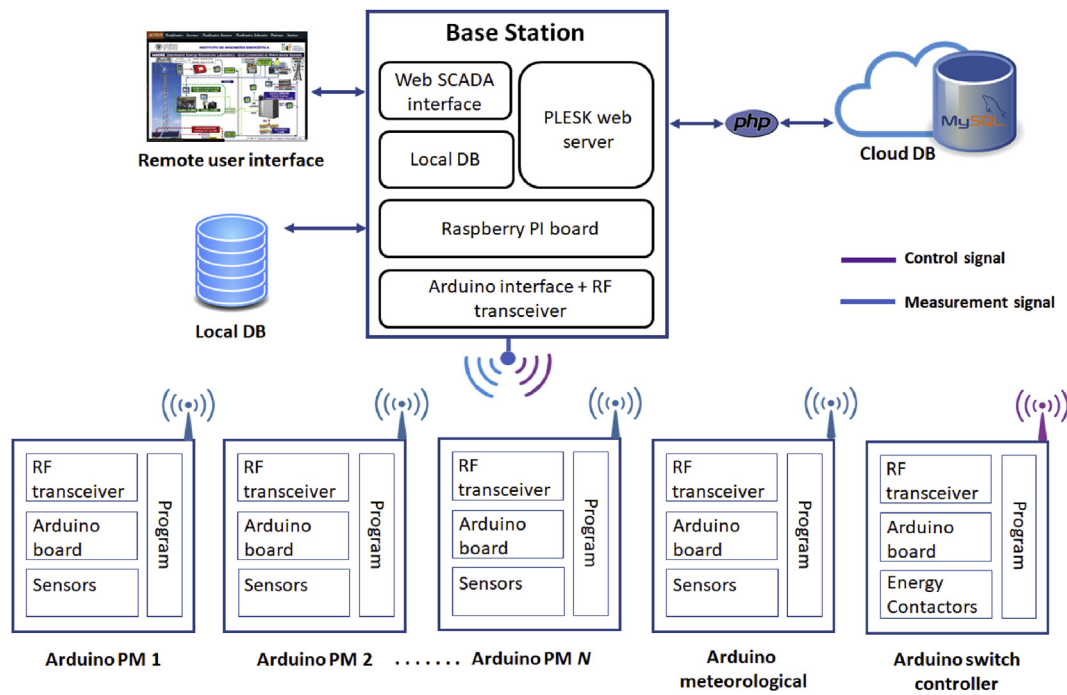
Fig. 8. Communications structure.
