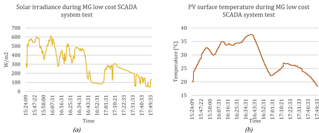
Fig. 14. (a) Solar irradiance (b) PV surface temperature data collecting for a short-term test of the LC-SCADA system.
