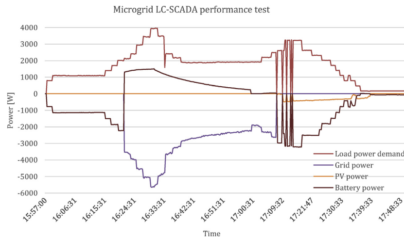
Fig. 13. LC-SCADA system data acquisition test over the microgrid.
