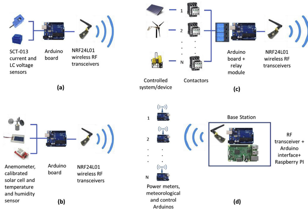
Fig. 7. Scheme of the Arduino wireless devices (a) Arduino wireless power meter (AWPM); (b) Arduino wireless meteorological data collector AWMDC; (c) Arduino wireless switch controller (AWSC); (d) Arduino-Raspberry Pi 3 wireless base station (ARWBS).
