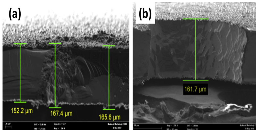
Fig. 6. Cross-sectional SEM pictures of patterns for (a)trench and (b)thru-hole.
