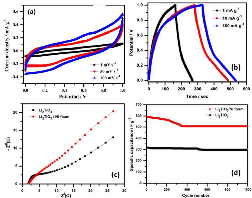
Fig. 5. (a) Cyclic voltammograms of \text{Li}_2\text{TiO}_3/\text{Ni} foam composite negatrod. (b) Charge-discharge curves \text{Li}_2\text{TiO}_3/\text{Ni} foam composite negatrod in asymmetric capacitor. (c) Nyquist plots of \text{Li}_2\text{TiO}_3/\text{Ni} foam composite negatrod and pristine \text{Li}_2\text{TiO}_3 negatrod in asymmetric capacitor. (d) Cycling performance of \text{Li}_2\text{TiO}_3/\text{Ni} foam composite negatrod and pristine \text{Li}_2\text{TiO}_3 negatrod in asymmetric capacitor.
