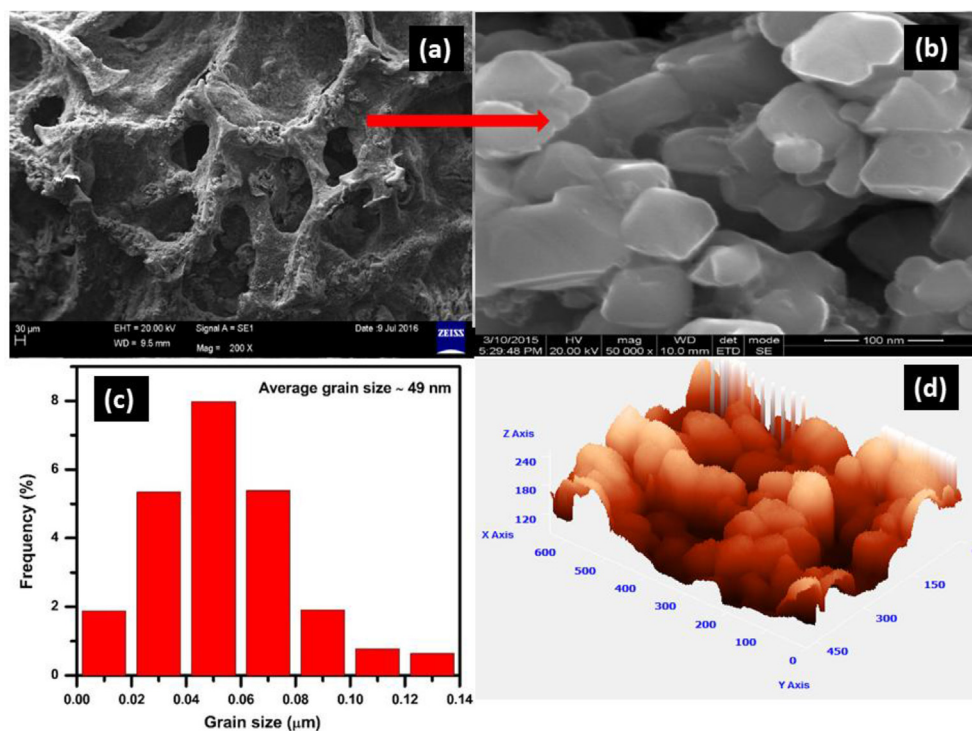
Fig. 2. (a) SEM image of \text{Li}_2\text{TiO}_3/\text{Ni} foam composite, (b) FESEM image of \text{Li}_2\text{TiO}_3 nano particles on Ni foam, (c) Particle size distribution determined from FESEM image and (d) 3D-surface topography of \text{Li}_2\text{TiO}_3 nanoparticles. This image was treated via the “image NOVA” software, which generated the z-axis from FESEM data. Numbers are in nm.
