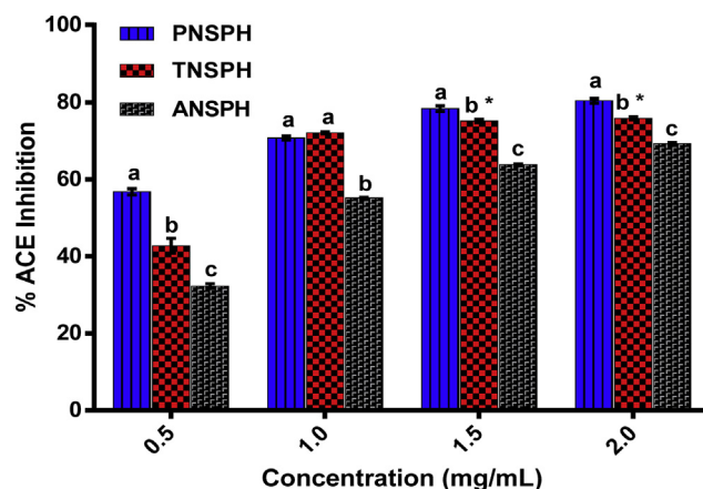
Fig. 3. ACE-inhibitory activity of pepsin, trypsin and Alcalase NSPHs. Values represent mean of triplicate determinations \pm SD. Different letters (abc) denote significant difference ( p < 0.05 ) among different samples at the same concentration. Bars with asterisk (*) denote insignificant difference ( p > 0.05 ) of the same sample at different concentrations. PNSPH – Pepsin Neem Seed Protein Hydrolysate; TNSPH – Trypsin Neem Seed Protein Hydrolysate; ANSPH – Alcalase Neem Seed Protein Hydrolysate.
