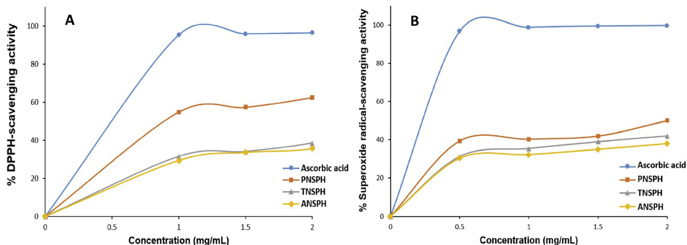
Fig. 1. DPPH-scavenging (A) and superoxide radical-scavenging (B) activities of pepsin, trypsin and Alcalase NSPHs. PNSPH – Pepsin Neem Seed Protein Hydrolysate; TNSPH – Trypsin Neem Seed Protein Hydrolysate; ANSPH – Alcalase Neem Seed Protein Hydrolysate.
