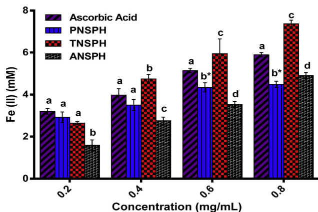
Fig. 2. Ferric-reducing power of pepsin, trypsin and Alcalase NSPHs. Values represent mean of triplicate determinations \pm SD. Different letters (a–d) denote significant difference ( p < 0.05 ) among different samples at the same concentration. Bars with asterisk (*) denote insignificant difference ( p > 0.05 ) of the same sample at different concentrations. PNSPH – Pepsin Neem Seed Protein Hydrolysate; TNSPH – Trypsin Neem Seed Protein Hydrolysate; ANSPH – Alcalase Neem Seed Protein Hydrolysate.
