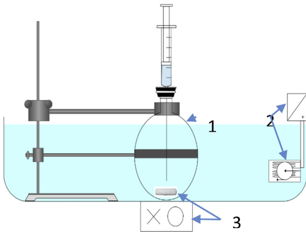
Fig. 2. Experimental setup.
