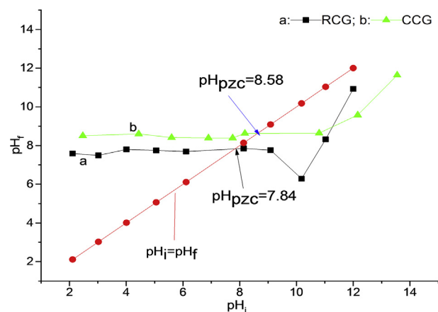
Fig. 5. \text{pH}_{pzc} of RCG (a) and CCG (b).
