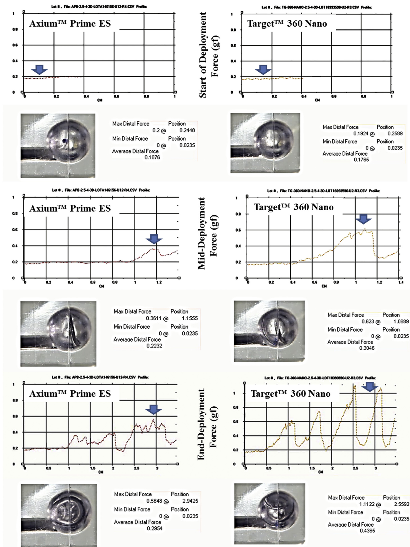
Fig. 2. Sequential deployment of the Axiom Prime ES and Target Nano coils inside the aneurysm. Force measured is shown for initial, mid-deployment and end-deployment stages, together with the corresponding video image of the coil at each stage.
