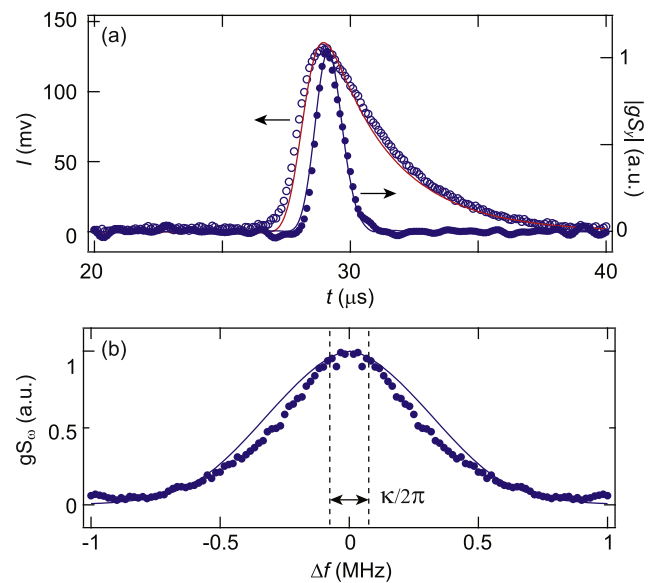
Fig. 4. (a) Quadrature signal of the emitted echo (open circles) and its effective spin component gS_y obtained by de-convolution of the cavity response (filled circles). The measurement is acquired with a repetition time of t_r = 1 s. (b) Fast Fourier transform of gS_y showing the spectral bandwidth of the echo, much larger than the cavity bandwidth \kappa/2\pi . Solid lines are numerical simulations.
