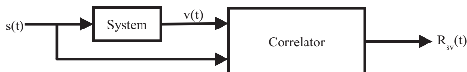
Fig. 1. A pseudorandom noise excitation, s(t) , stimulates the System and produces a response, v(t) . The resulting correlation of these signals, R_{sv}(t) , is proportional to the impulse response of System.
