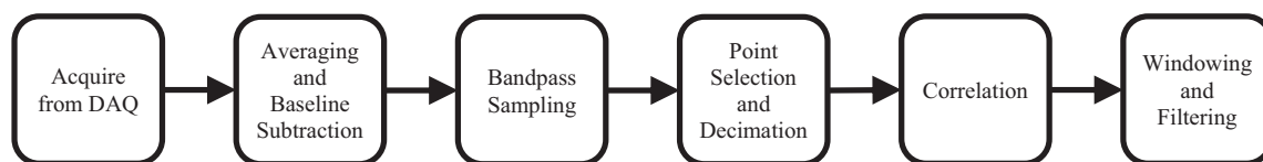
Fig. 7. Block diagram of processing steps in the acquisition software. After acquisition, the first waveform represents the baseline. This waveform is subtracted from all other acquired waveforms. After baseline subtraction, the data is resampled using quadrature bandpass sampling. A set of 256 equally spaced points are extracted from the data and correlated with the original stochastic sequence to generate the FID. A last stage of filtering produces the final result.
