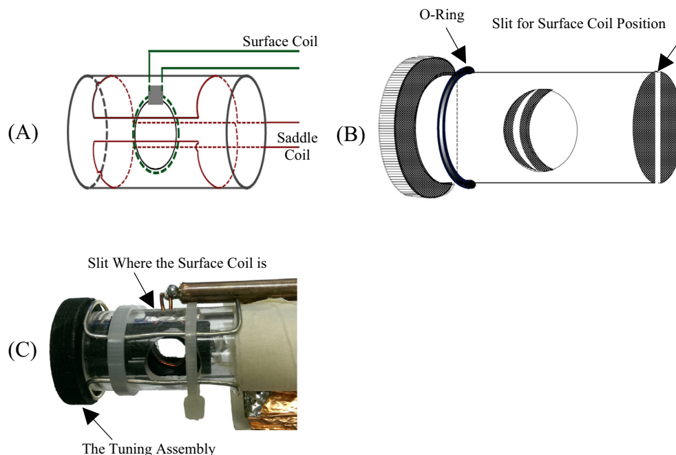
Fig. 4. (A) Schematic of a crossed resonator with saddle transmit and an inner surface coil receive pair. (B) The tuning assembly. The mechanism is of a PVC insert fabricated with a slit in the middle. The diameter of the insert is the inner diameter of the Lucite tube. The slit width is equal to the diameter of the surface coil wire. In the assembly, an O-ring is positioned in such a way, once the tuning assembly is inserted, it will hold tightly. Since the surface coil is inside the slit, the position can be changed by tuning the assembly. (C) The actual resonator assembly.
