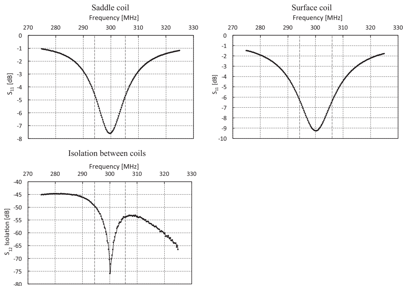
Fig. 5. Frequency response of each coil and the measured isolation between the two coils with a center frequency of \sim 300 MHz and a 3 dB bandwidth of \sim 12 MHz for each coil. The isolation ranges from \sim 50 dB at the bandwidth boundaries to -76 dB at the center. All readings are taken using Rohde & Schwarz Vector Network Analyzer – ZNC3.
