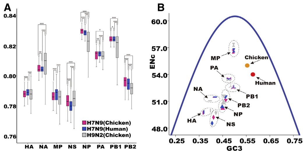
Fig. 1. (A) Codon adaptation index (CAI) analysis of all eight H7N9 and H9N2 AIV genes to their hosts. Chicken-isolated H7N9 AIVs are shown in red, human-isolated H7N9 in blue, and chicken-isolated H9N2 in grey. (B) ENC denotes the effective number of codons, and GC3 denotes the GC content on the third position of synonymous codons. The solid blue line represents the expected curve derived from the positions of strains if codon usage was only determined by GC3 composition (i.e., without selection). Points on or close to the curve means that the bias was caused by mutation pressure, otherwise, the varied positions are due to natural selection or other factors.
