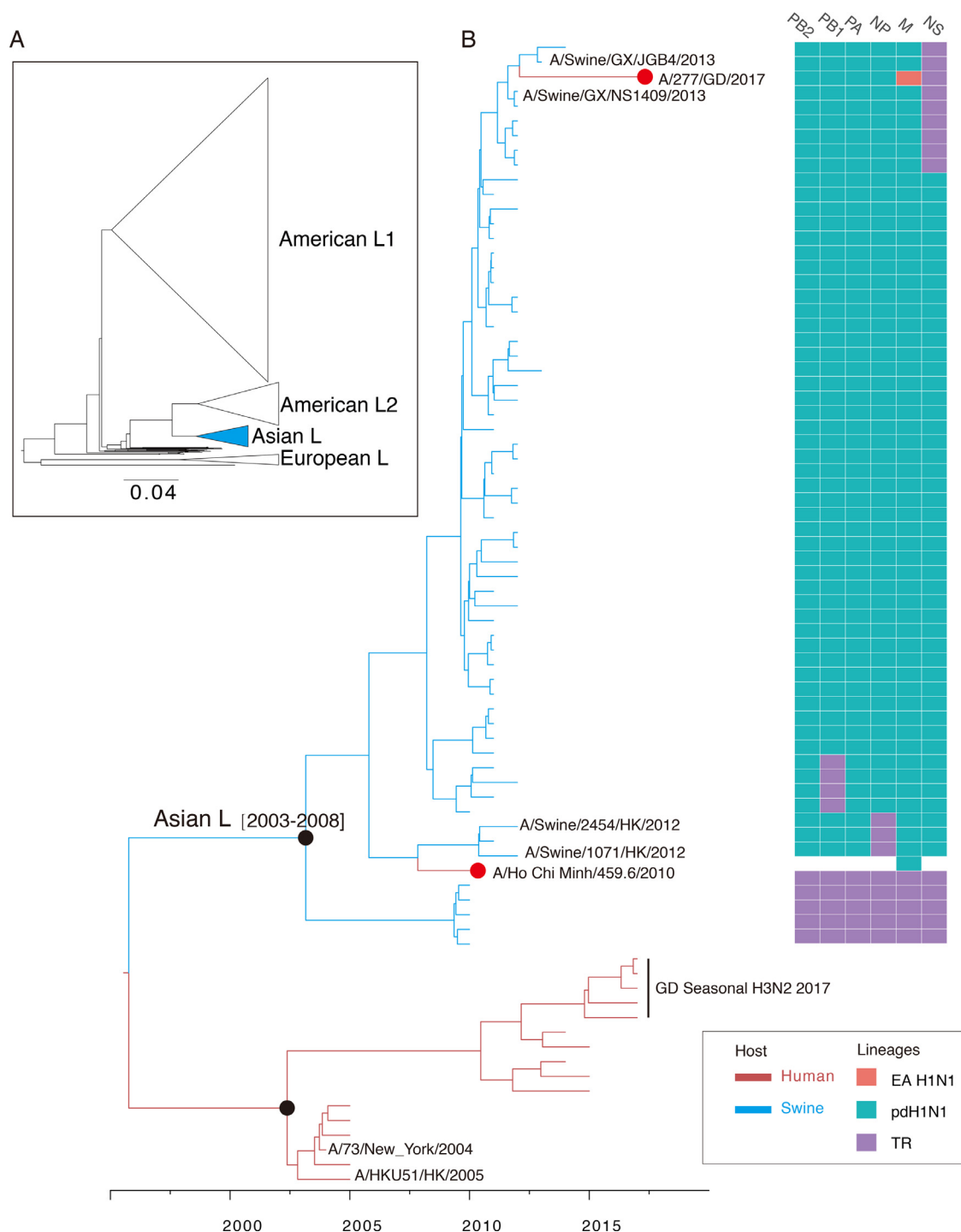
Fig. 1. Phylogenetic analyses of the HA gene segment. (A) Maximum likelihood (ML) tree inferred from swine H3N2 viruses collected in 2012–2017. Phylogenetic lineages were named according to the locations of lineage strains (Fig. S1A). The Asian lineage (Asian L) was highlighted with blue. (B) Bayesian Maximum Clade Credibility (MCC) tree of HA gene inferred from swine H3N2 viruses and closely related human H3N2 viruses. Branch colors represented the most probable ancestral species. A/GD/277/H3N2/2017 and A/Ho Chi Minh/459.6/2010 clinical strains were highlighted with red dots, and their closely related sequences were also marked. The combination of internal genes for A/GD/277/H3N2/2017 and closely related strains were shown on the right of MCC tree. Black circles indicate posterior support >0.95. EA H1N1: Europe-avian like H1N1; pdH1N1: 2009 pandemic H1N1 virus; TR: Triple Reassortant H3N2 virus.
