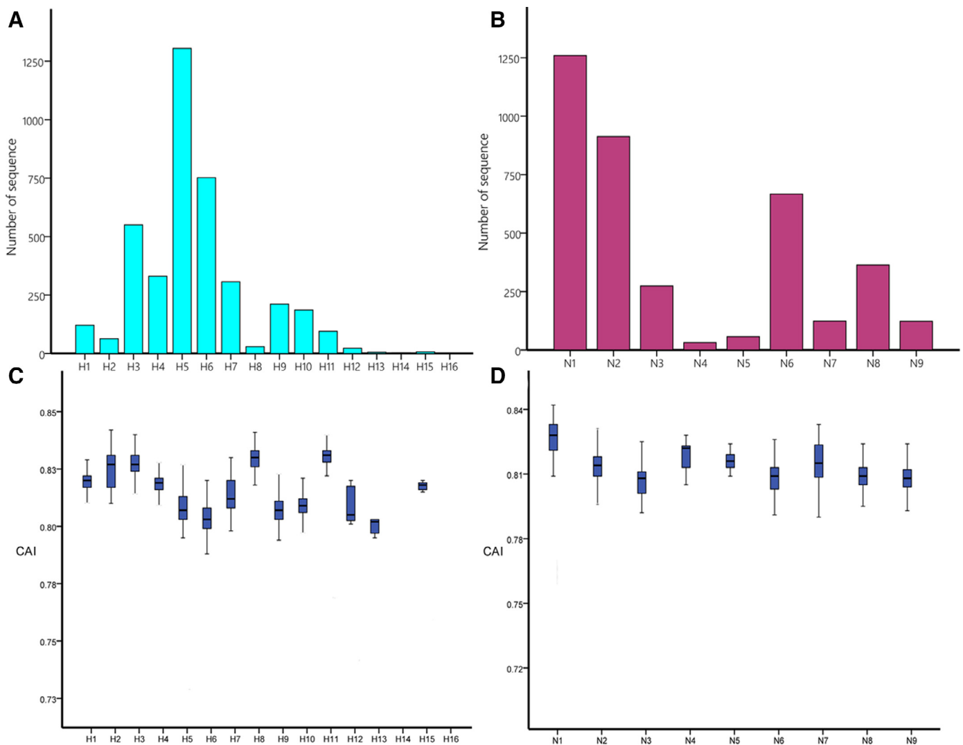
Fig. 1. (A) The abundance of 16 HA subtypes of avian influenza viruses isolated from ducks. (B) The abundance of 9 NA subtypes of avian influenza viruses isolated from ducks. (C) Codon adaptation index (CAI) of 16 HA subtypes. (D) Codon adaptation index (CAI) of 9 NA subtypes. All available sequences of each subtype were collected from NCBI Influenza Virus Resource.
