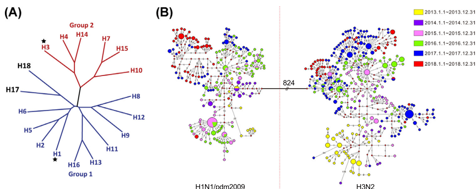
Fig. 1. Phylogenetic relationships of human H3N2 and H1N1/pdm2009 IAVs. (A) Phylogenetic tree of the 18 HA genes. This figure was modified from Wu et al study. (B) Phylogenetic network of HA gene for human H3N2 and H1N1/pdm2009 IAVs. The numbers on the lines represent the numbers of the nucleotide substitutions.
