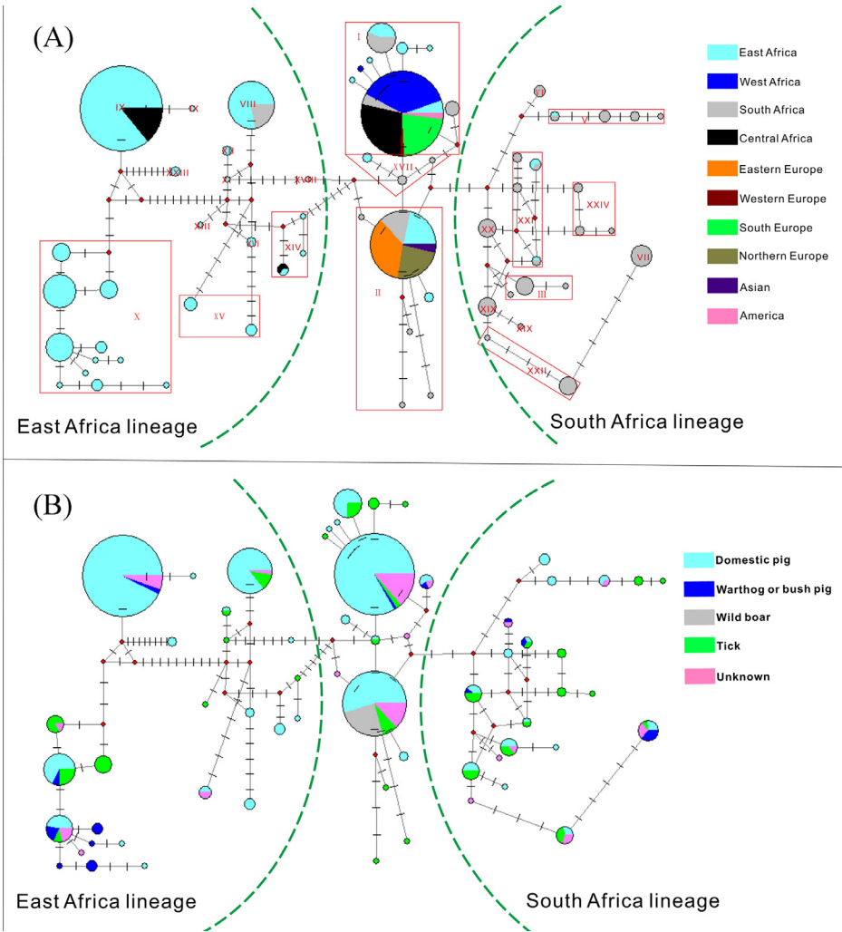
Fig. 1. Phylogenetic network for the p72 gene from ASFV. (A) Phylogenetic network displaying the geographical distribution of where the viruses were isolated. (B) Phylogenetic network marked for host information.
