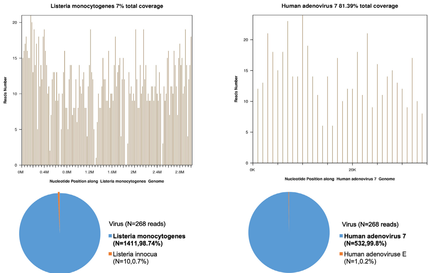
Fig. 2. Next-generation sequencing of listeria monocytogenes and adenovirus.
