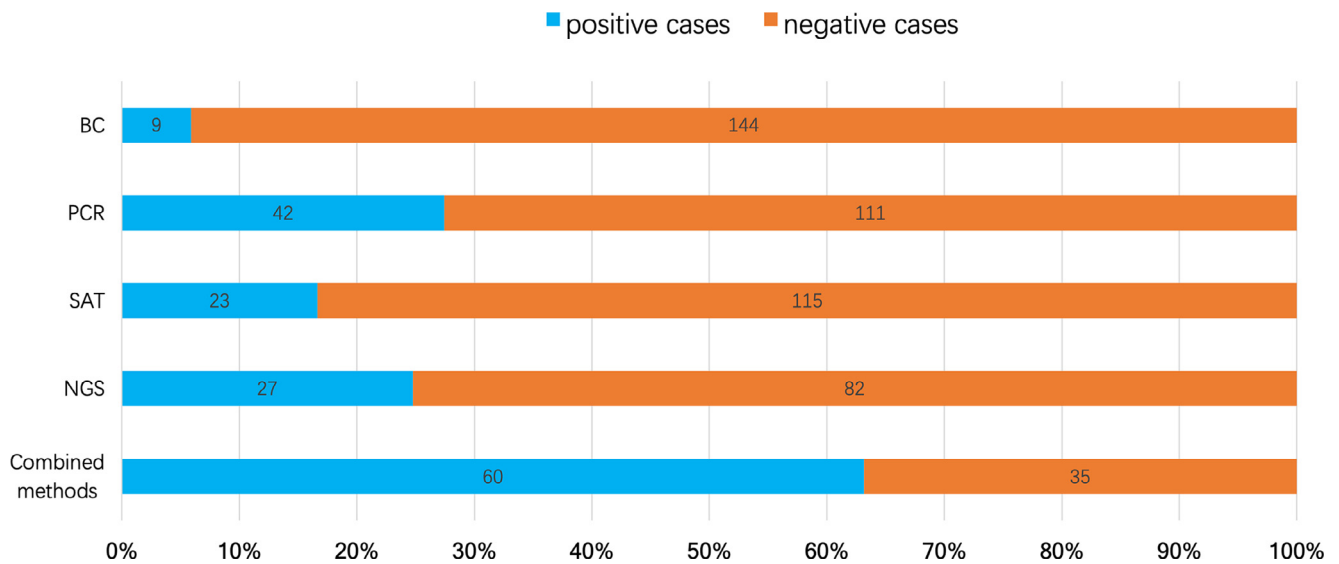
Fig. 1. NGS (next-generation sequencing), SAT (simultaneous amplification and testing), BC(bacterial culture).
