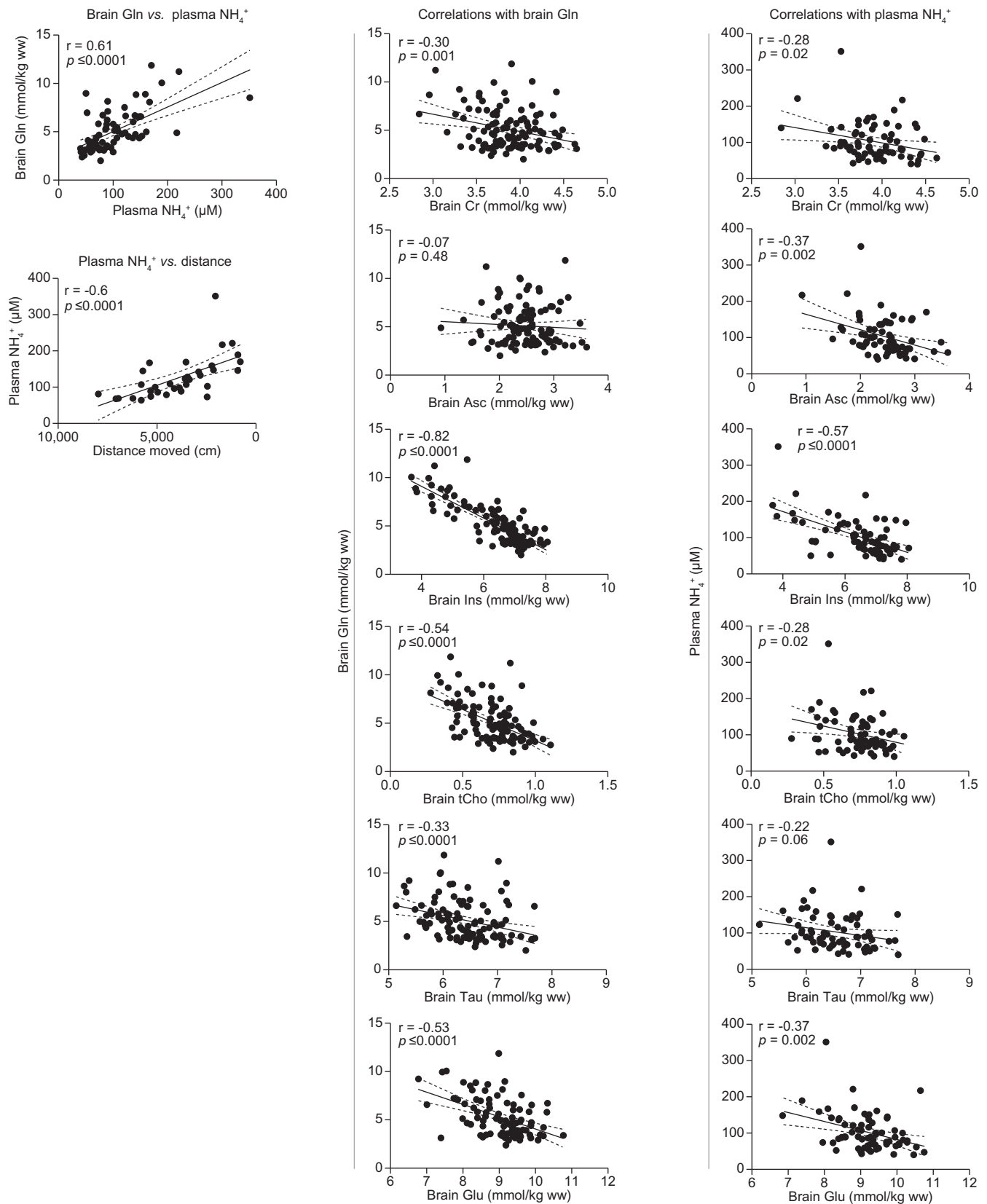
Fig. 6. Pearson correlations between plasma \text{NH}_4^+ , brain metabolites and distance moved over the duration of the entire study. Pearson correlation coefficients ( r ) and corresponding p values are shown together with 95% confidence bands (dotted lines) surrounding the best-fit line (linear regression). All the longitudinally acquired data were used. Asc, ascorbate; Cr, creatine; Gln, glutamine; Glu, glutamate; GPC, glycerophosphocholine; Ins, myo inositol; PCho, phosphocholine; Tau, taurine; tCho, total choline (GPC + PCho).
