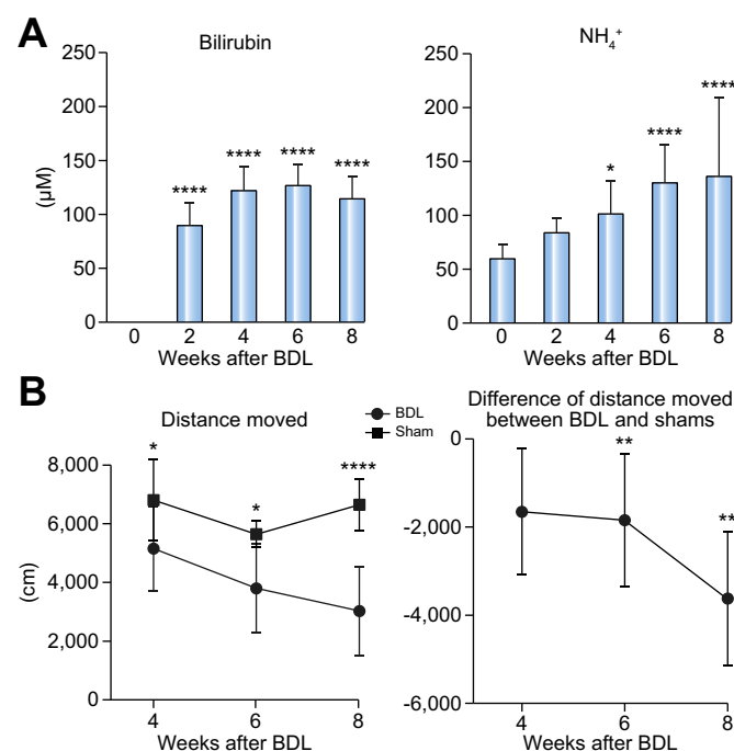
Fig. 1. BDL-induced changes in plasma total bilirubin, \text{NH}_4^+ and distanced travelled. (A) Longitudinal changes of plasma total bilirubin and \text{NH}_4^+ . Bilirubin was non-measurable before BDL. (B) Distance travelled by BDL and sham-operated rats. Mean \pm SD. Significance level between weeks 0 and 2–8: * p < 0.05, ** p < 0.01, *** p < 0.001, **** p < 0.0001 (1-way [plasma] and 2-way [distance] ANOVA). BDL, bile-duct ligation.
