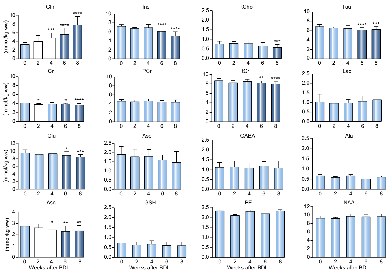
Fig. 3. Longitudinal ^1\text{H} -MRS data of the main brain metabolites from 0 to 8 weeks post-BDL. Mean \pm SD, significance level between weeks 0 and 2–8: * p < 0.05, ** p < 0.01, *** p < 0.001, **** p < 0.0001 (1-way ANOVA), metabolite concentrations at week 0 and those of metabolites showing non-significant changes are shown in light blue, while the early changes are shown in white and late changes in dark blue. ^1\text{H} -MRS, proton magnetic resonance spectroscopy; Ala, alanine; Asc, ascorbate; Asp, aspartate; BDL, bile-duct ligation; Cr, creatine; GABA, \gamma aminobutyric acid; Glc, glucose; Gln, glutamine; Glu, glutamate; GPC, glycerophosphocholine; GSH, glutathione; Ins, myo inositol; Lac, lactate; NAA, N acetylaspartate; NAAG, N acetylaspartylglutamate; PCho, phosphocholine; PCr, phosphocreatine; PE, phosphoethanolamine; Tau, taurine; tCho, total choline (GPC + PCho); tCr, total creatine (Cr + PCr).
