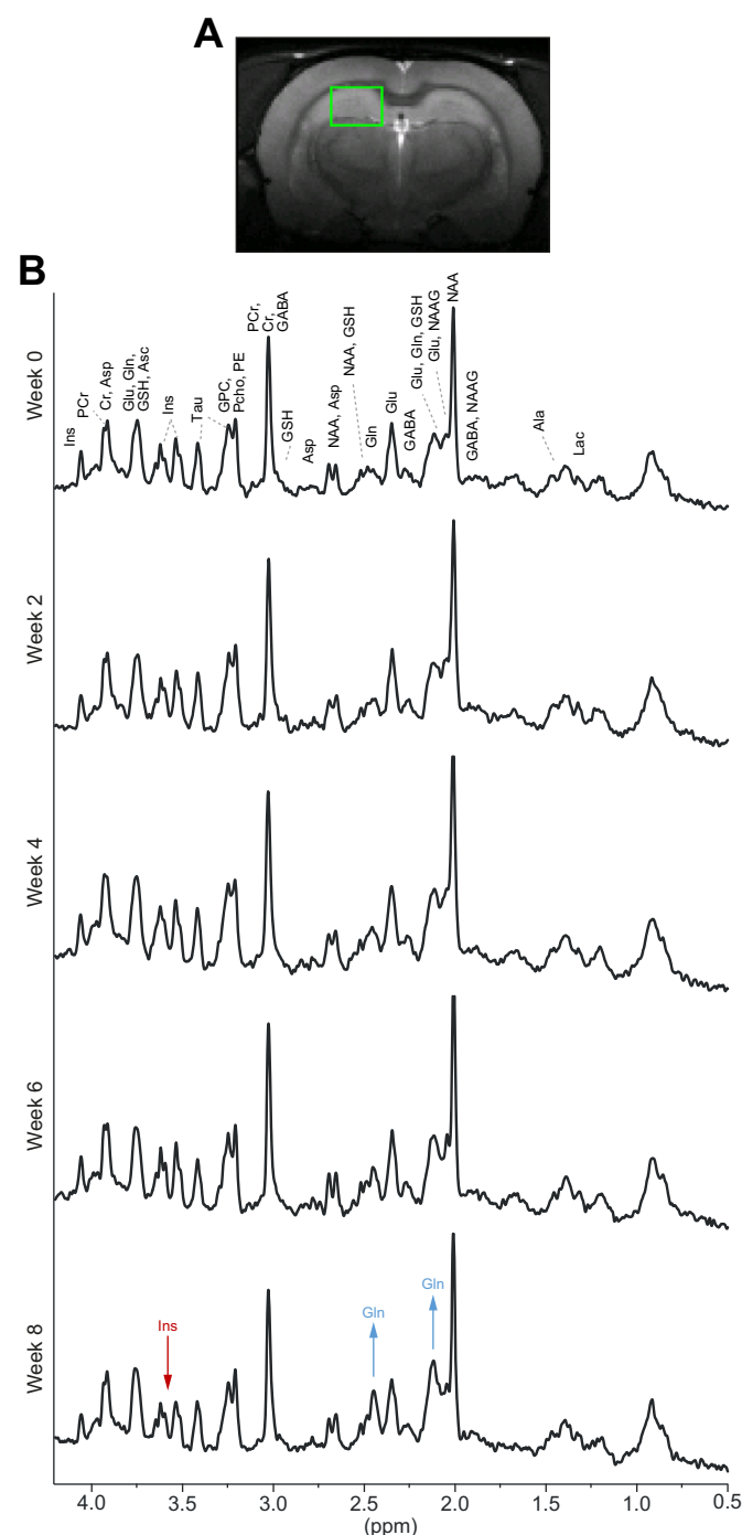
Fig. 2. Representative in vivo ^1\text{H} -MRS spectra acquired longitudinally in 1 BDL rat at 9.4T: (A) Anatomical \text{T}_2 weighted image showing the hippocampus ^1\text{H} -MRS voxel (green). (B) Brain ^1\text{H} -MRS spectra measured before BDL and at post-operative weeks 2–8; Gln increase and Ins decrease is clearly visible. ^1\text{H} -MRS, proton magnetic resonance spectroscopy; Ala, alanine; Asp, aspartate; BDL, bile-duct ligation; Cr, creatine; GABA, \gamma aminobutyric acid; Glc, glucose; Gln, glutamine; Glu, glutamate; GPC, glycerophosphocholine; GSH, glutathione; Ins, myo inositol; Lac, lactate; NAA, N acetylaspartate; NAAAG, N acetylaspartylglutamate; PCho, phosphocholine; PCr, phosphocreatine; PE, phosphoethanolamine; Tau, taurine. (This figure appears in colour on the web.)
