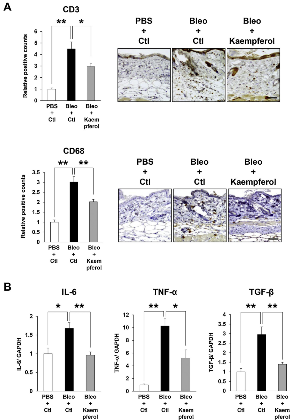
Fig. 3. Kaempferol suppressed the amount of inflammatory cells and the inflammatory and pro-fibrotic cytokines in the skin of bleomycin-treated mice in vivo . (A) The number of infiltrating CD3 + T cells and CD68 + macrophages in the dermis was determined by counting cells. Representative images of CD3 and CD68 staining in the skin. Values were determined in six random microscopic fields in n = 4-6 mice per groups. Scale bar = 50 \mu m. (B) mRNA levels of inflammatory and pro-fibrotic cytokines, IL-6, TNF- \alpha and TGF- \beta in the skin treated with subcutaneous injections of bleomycin of control PBS, and treated with intraperitoneal injection of kaempferol or control DMSO for 5 days. n = 4-8 mice in each group. The number of cells or mRNA levels in control mice were assigned values of 1. Values represent mean \pm SEM. * P < 0.05 , ** P < 0.01 .
