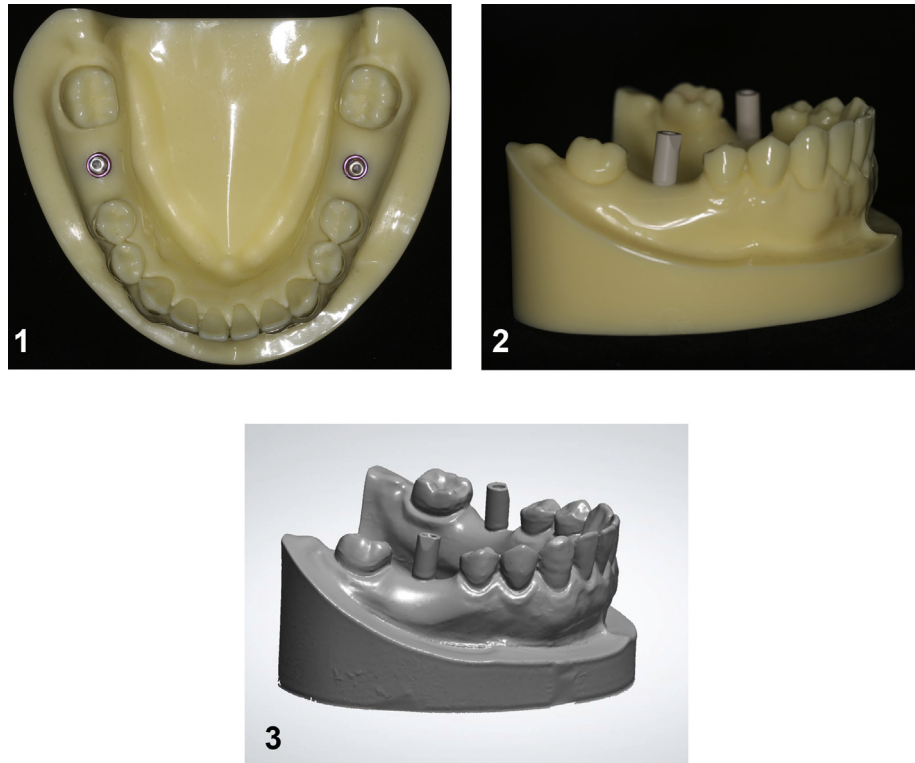
Fig. 5. 1. Placing of implants on the model, 2. The scan bodies are screwed onto the implants, 3. 3D view of the postoperative optical model scan.
