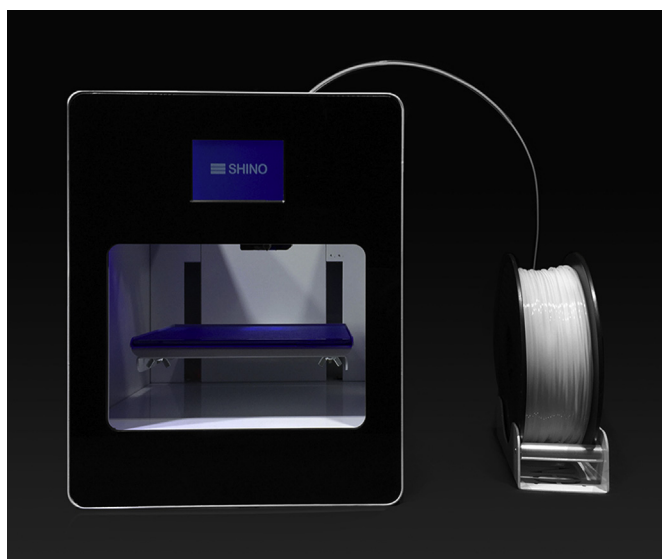
Fig. 3. FDM printer (Lingtong III, Beijing SHINO, China).
