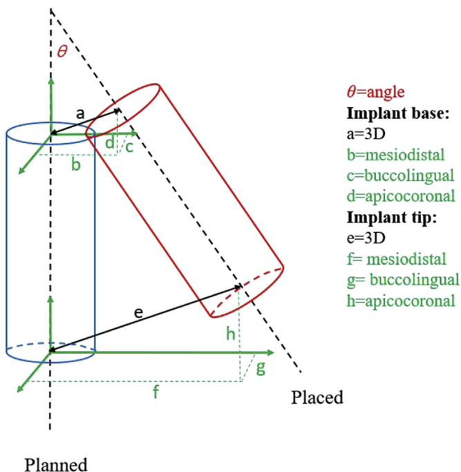
Fig. 6. Schematic diagram of accuracy evaluation. The position of the placed (red) implant was compared with that of the planned (blue) implant.
