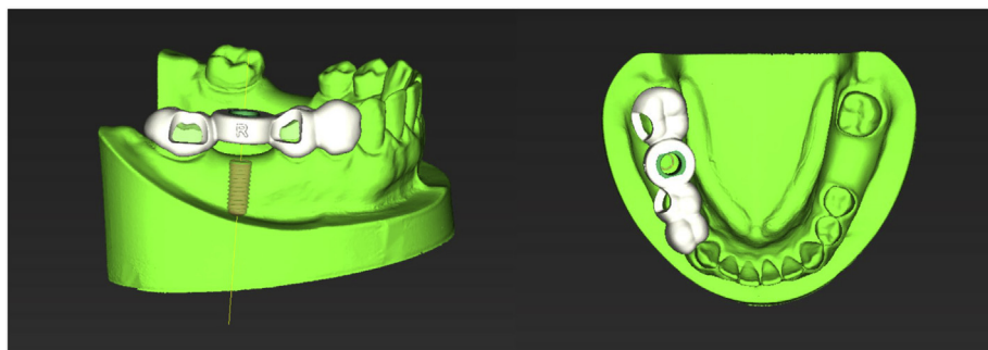
Fig. 2. The implant position for tooth 46 and view of the surgical template resting on the adjacent teeth.
