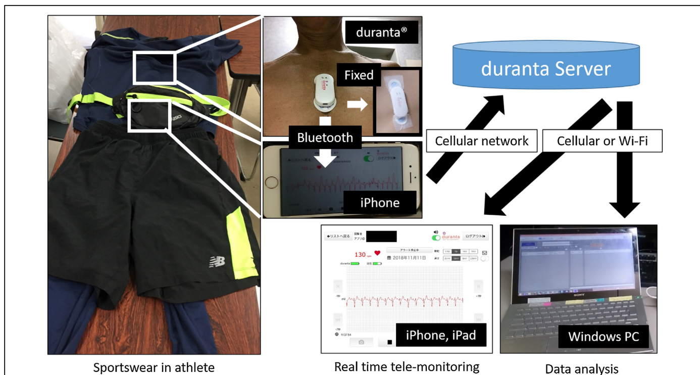
Fig. 1. Overview of the electrographic tele-monitoring system by duranta ® in athlete. The main body of the device is placed on the chest, which is connected to an iPhone through Bluetooth. Acquired electrocardiogram waves are transferred to the cloud server, via 3G/4G/LTE network. Real-time tele-monitoring data is available using both an iPhone and an iPad via the network, whereas detailed data analysis is achieved by a personal computer with Windows OS.
