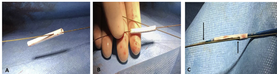
Fig. 2. Pictures showing inflated covered stent (A) with a small hole made across the polytetrafluoroethylene layer, and the first wire placed inside. (B) The second wire inserted longitudinally inside the main stent lumen. (C) The stent re-crimped on the balloon, with the wires forming a double rail (black arrows) before insertion into the 12 Fr sheath. In this way, continued access to both branches is maintained and a second stent could be advanced at the level of the bifurcation to preserve side branch patency, if needed.
