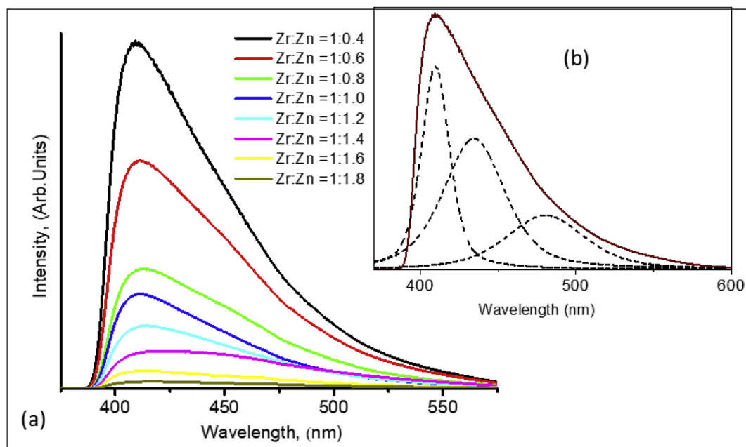
Figure 6. (a) Emission spectrum of the composite at varying ratios of the precursors while inset (b) is the deconvoluted \text{Zr:Zn} = 1:0.4 profile showing peaks at 409, 434 and 480 nm.
