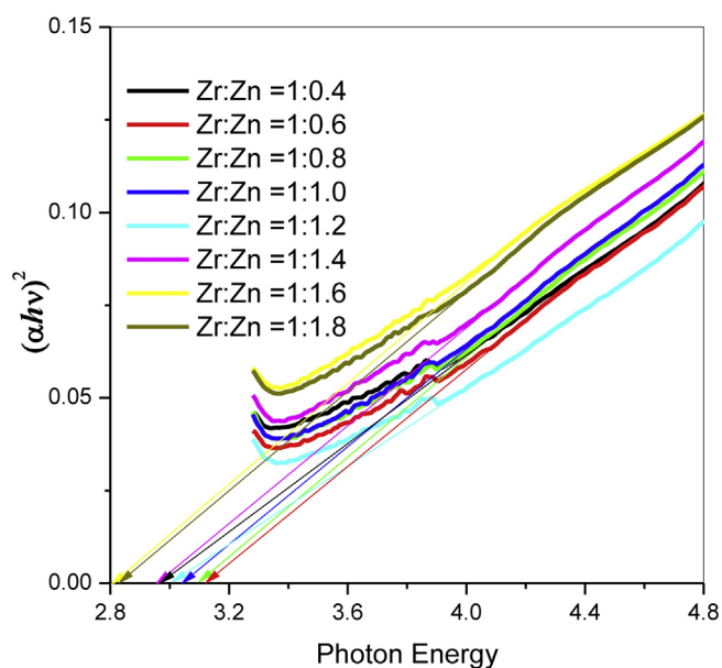
Figure 8. Kubelka-Munk function of the composite for determining energy bandgap.
