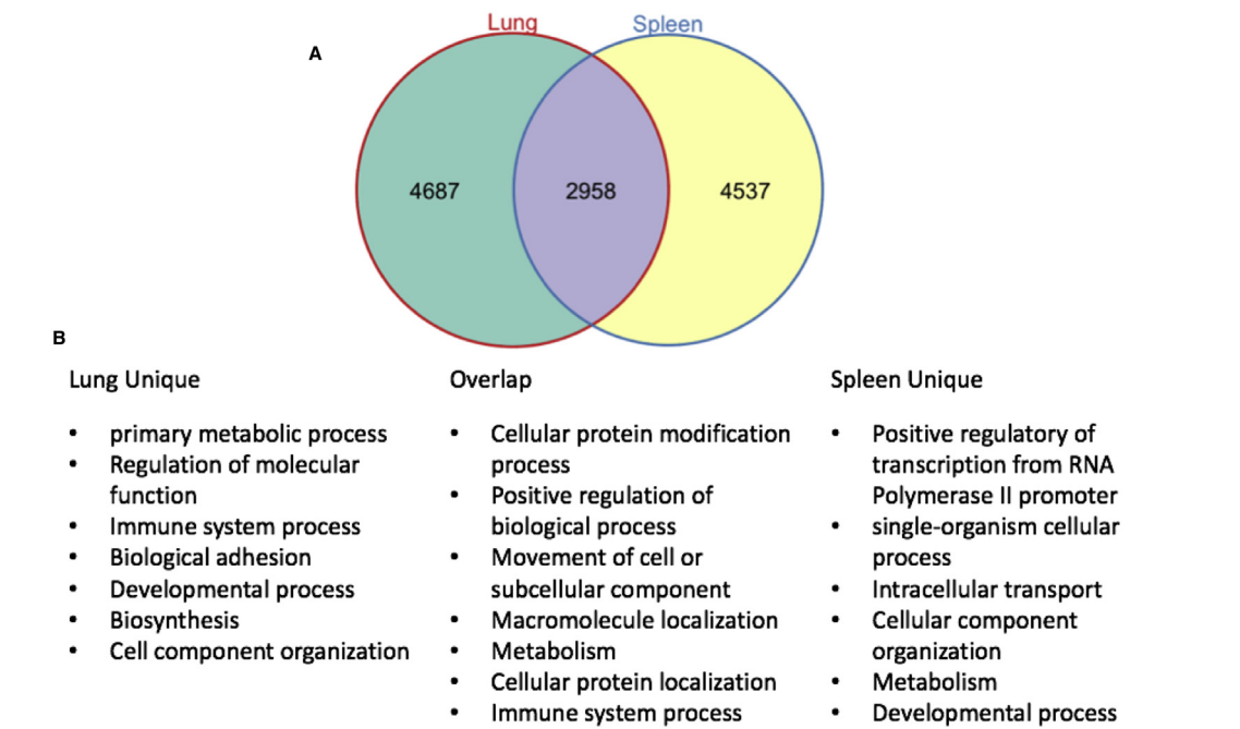
Fig. 1. The differences of the gene ontology enrichment of DRGs between spleen and lung. A. The Venn diagram for the number of significant DRGs in the lung and spleen. B. The significant gene ontology terms for each group of genes.
