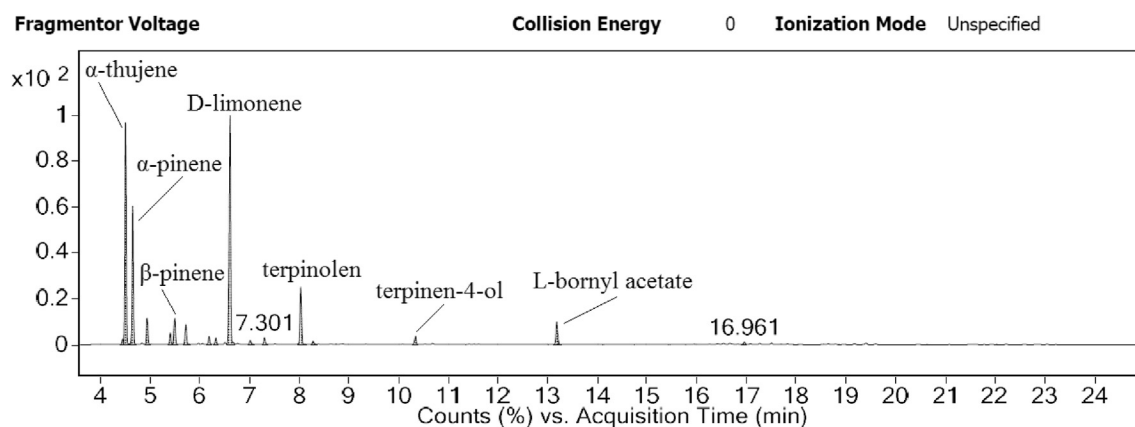
Fig. 4. GC-MS chromatogram of FPC.
