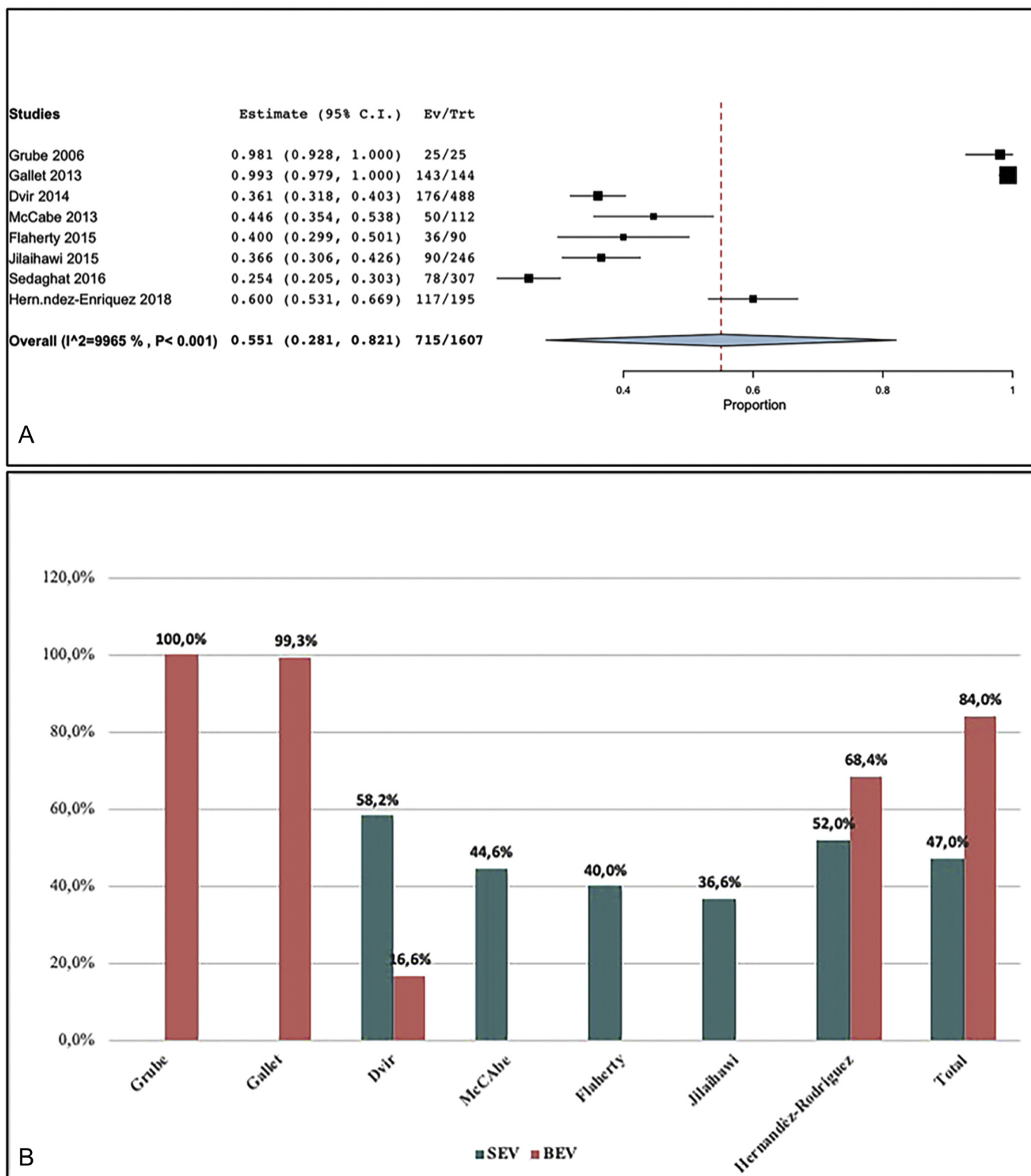
Fig. 4. A) Pooled prevalence of thrombocytopenia in TAVI patients. B) Patients that experienced thrombocytopenia after balloon-expandable and self-expandable trans-catheter aortic valves implantation.
