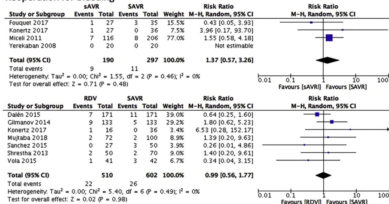
Fig. 2. Forrest plots showing pooled effect estimated from random-effects models comparing stentless vs. stented aortic tissue valves and rapid deployment vs. stented tissue valves for post-operative platelet count (A), red blood cell transfusion (B), and reoperation for bleeding (C).
