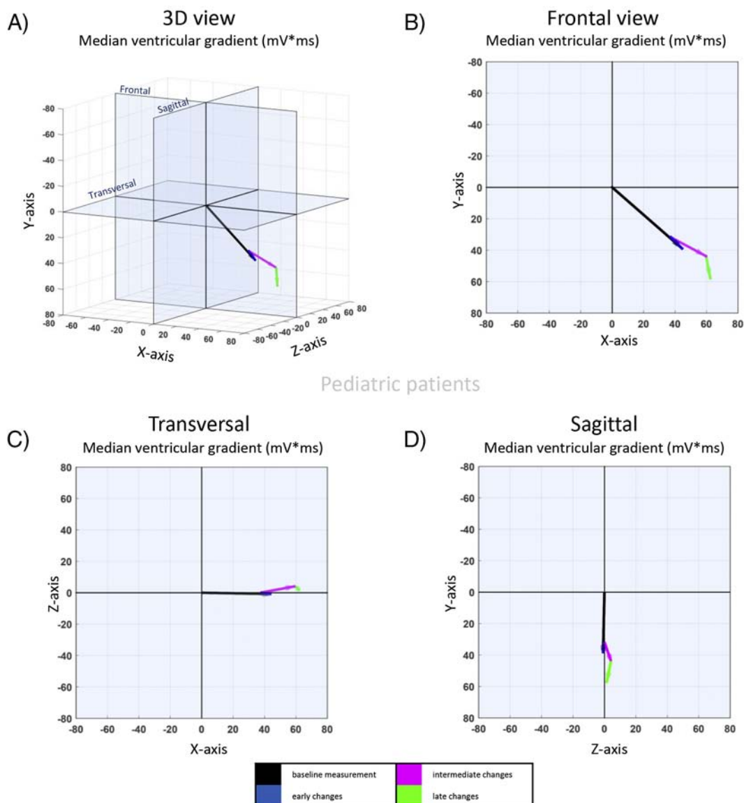
Fig. 1. Spatial changes of the median ventricular gradient in the pediatric patients. A) Three-dimensional (3D) view of the VG changes. B) Frontal view. C) Transversal view. D) Sagittal view. In all images the black line represents the baseline measurement, the blue line represents the early changes, the purple line represents the intermediate changes, and the green line represents the late changes.
