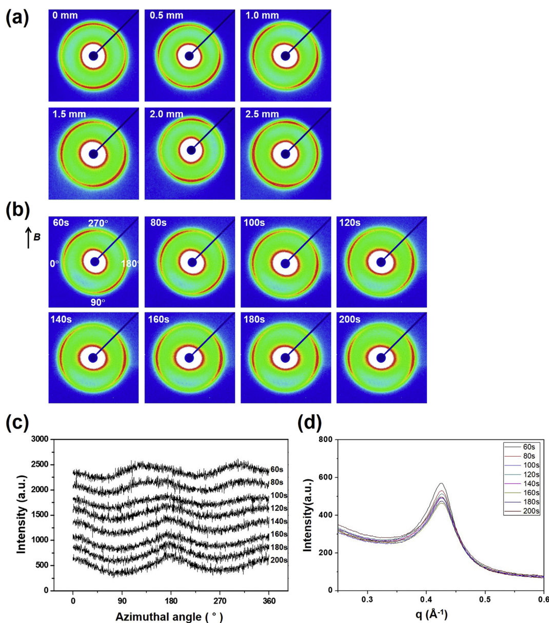
Fig. 4. (a) SAXS images of M-M3 when measuring point of the X-ray changes every 0.5 mm. (b) Change in SAXS images of M-M3 sample over time under a magnetic field. (c) Azimuthal scattering intensity of the M-M3 sample over time under a magnetic field. (d) 1-D scattering intensity profiles of the M-M3 sample over time under magnetic field.
