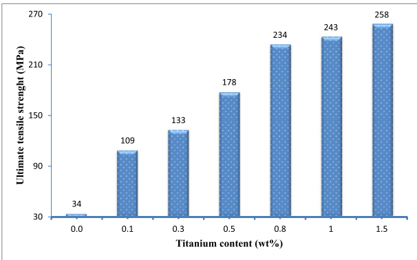
Fig. 2. Effect of titanium content on the ultimate tensile strength of Cu–3Si–xTi alloy.
