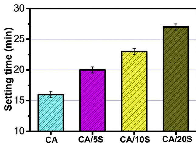
Fig. 3. The setting time values of CA cement containing 0, 5, 10 and 20 wt.% of nano-SiO 2 particles.
