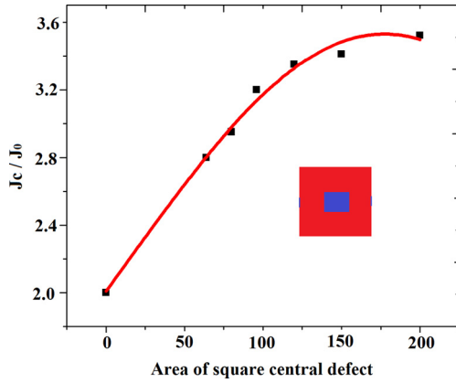
Fig. 14. Theoretical fitting for \bar{J}_c for different areas of a central square defect of area A , J_c = \exp(0.697 + 0.006A - 1.792A^2) .
