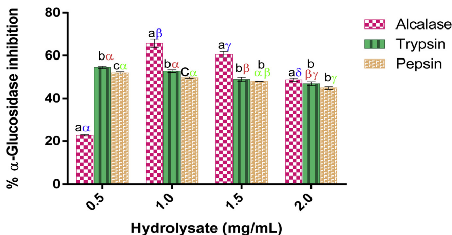
Fig. 3. \alpha -glucosidase- inhibitory effect of L. cylindrica seed protein hydrolysates. Each bar depicts the mean of three replicates determinations \pm SD. Bars at the same concentration but with different Latin letters (abcd) are significantly different at p < 0.05 . Bars of the same sample/enzyme at different concentrations with different Greek letters ( \alpha\beta\gamma\delta ) show significant difference at p < 0.05 .
