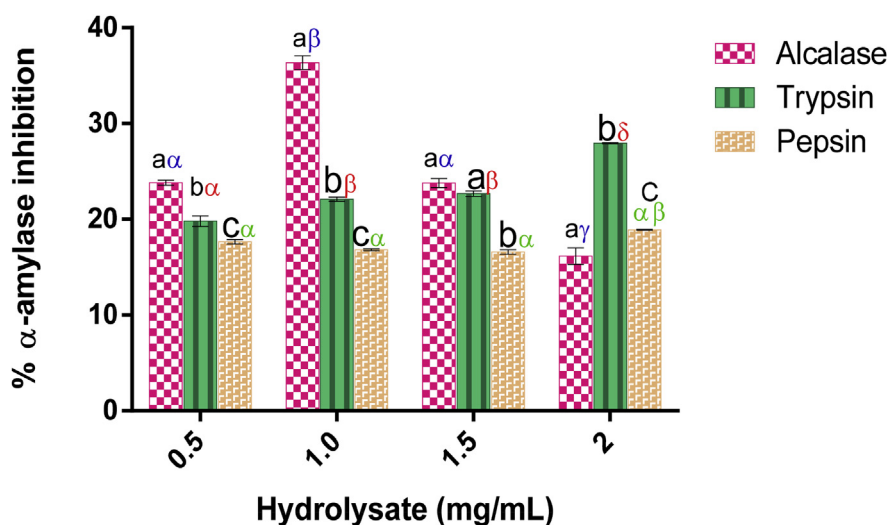
Fig. 2. \alpha -Amylase-inhibitory effect of L. cylindrical seed protein hydrolysates. Each bar depicts the mean of three replicates determinations \pm SD. Bars at the same concentration but with different Latin letters (abcd) are significantly different at p < 0.05 . Bars of the same sample/enzyme at different concentrations with different Greek letters ( \alpha\beta\gamma\delta ) show significant difference at p < 0.05 .
