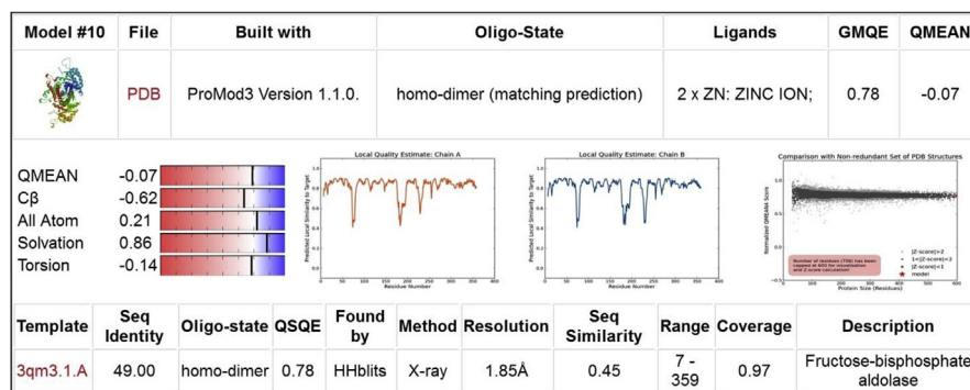
Fig. 7. Quality of the built model #10.
