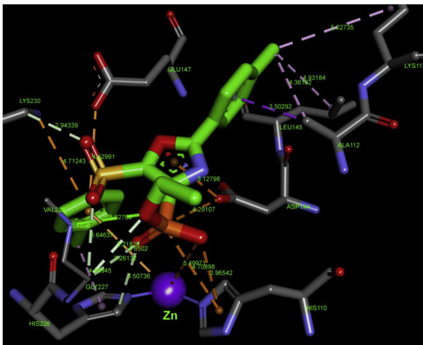
Fig. 16. Molecular docking of compound 6 into the active site of FBA-II C. albicans .
