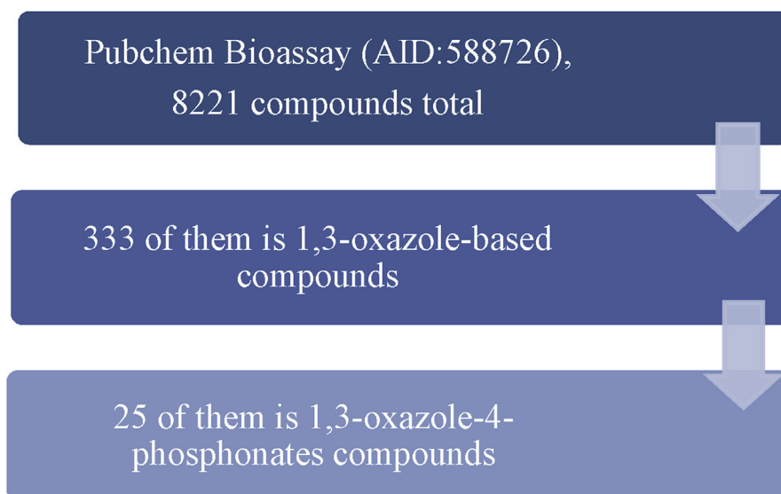
Fig. 3. Analysis of FBA-II M. tuberculosis inhibitors structures (PubChem bioassay AID: 588726). The structures of some FBA-II M. tuberculosis inhibitors from PubChem AID: 588726 are shown in Fig. 4.
