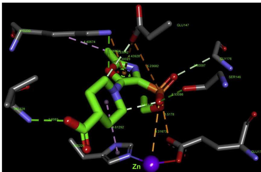
Fig. 17. Molecular docking of compound 1 into the active site of FBA-II C. albicans .
