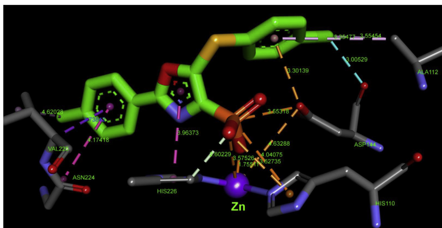
Fig. 14. Molecular docking of compound 4 into the FBA-II C. albicans active site.
