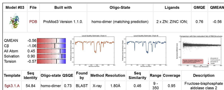
Fig. 9. Quality of the built model #03. In our opinion, model #10 is the most optimal considering the values of resolution (1.85Å), QMEAN (-0.07), GMQE (0.78), GSQE (0.78) indicators.
