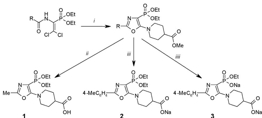
Scheme 1. Reagents and conditions: (i) methyl isonipecotinate/ \text{Et}_3\text{N}(\text{exc.})/\text{MeOH} , 3h, reflux. (ii) \text{R} = \text{Me} ; 1eq \text{NaOH}/\text{H}_2\text{O} , 30h, RT. (iii) \text{R} = 4\text{-MeC}_6\text{H}_4 ; 1. 1eq \text{NaOH}/\text{H}_2\text{O} , 30h, RT; 2. 1eq \text{NaHCO}_3/\text{H}_2\text{O} , RT. (iiii) \text{R} = 4\text{-MeC}_6\text{H}_4 ; 1. 4eq \text{NaOH}/\text{EtOH} , 10 days, RT; 2. 2eq \text{NaHCO}_3/\text{H}_2\text{O} , RT.
