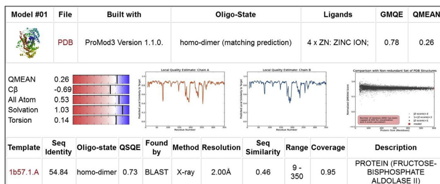
Fig. 8. Quality of the built model #01.
