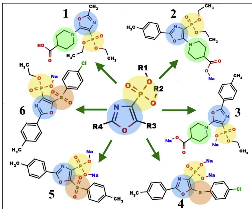
Fig. 5. Design of the 1,3-oxazole-4-phosphonate derivatives as active FBA-II C. albicans inhibitors.
