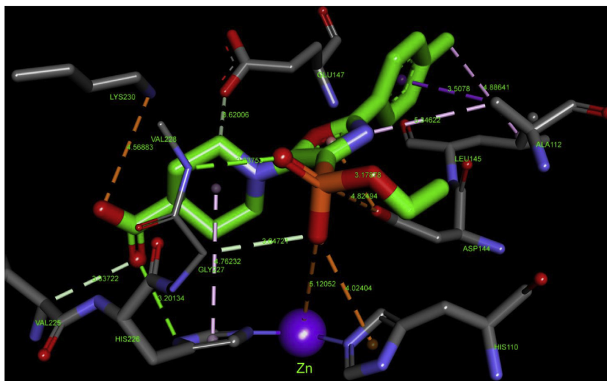
Fig. 13. Molecular docking of compound 3 into the active site of FBA-II C. albicans .
