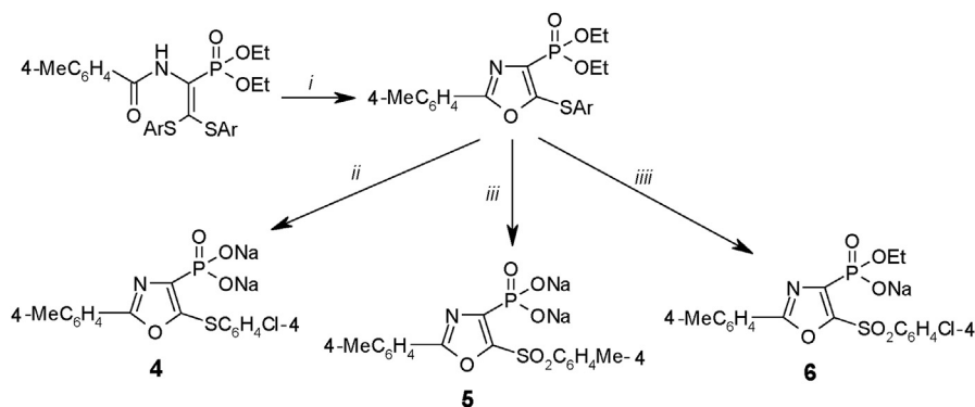
Scheme 2. Reagents and conditions: (i) \text{Ag}_2\text{CO}_3(\text{exc.})/\text{dioxan} , 8h, reflux; (ii) \text{Ar} = 4\text{-ClC}_6\text{H}_4 ; 1. \text{HBr}/\text{MeCOOH} , 6h, RT; 2. 2eq \text{NaHCO}_3/\text{H}_2\text{O} , RT; (iii) \text{Ar} = 4\text{-MeC}_6\text{H}_4 ; 1. \text{HBr}/\text{MeCOOH} , 6h, RT; 2. \text{H}_2\text{O}_2/\text{MeCOOH} , 2h, reflux; 3. 2eq \text{NaHCO}_3/\text{H}_2\text{O} , RT; (iiii) \text{Ar} = 4\text{-ClC}_6\text{H}_4 ; 1. \text{HBr}/\text{MeCOOH} , 6h, RT; 2. \text{H}_2\text{O}_2/\text{MeCOOH} , 2h, reflux; 3. 1eq \text{NaHCO}_3/\text{H}_2\text{O} , RT.
