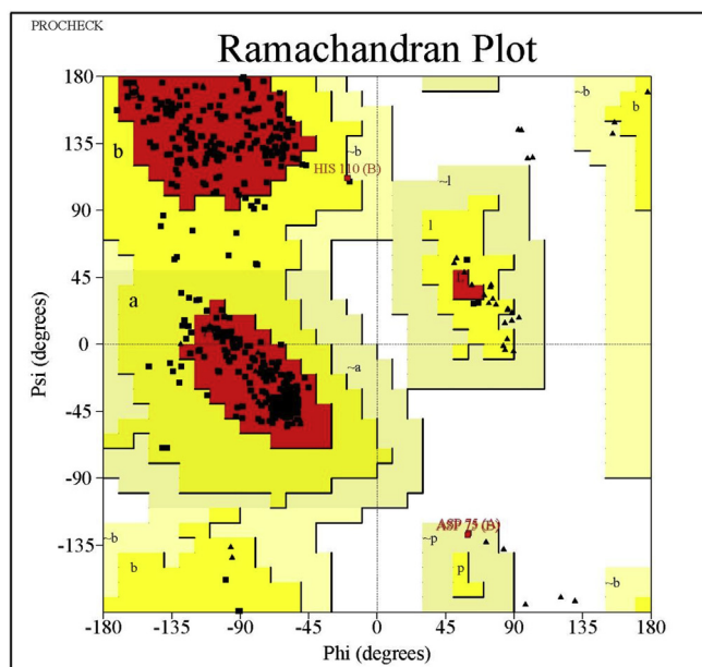
Fig. 12. Ramachandran plot of the stereochemical quality of FBA II C.albicans model generated by PROCHECK validation server.
