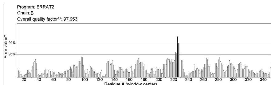
Fig. 11. The 3D profile of subunit B FBA-II C.albicans verified by using ERRAT server.
