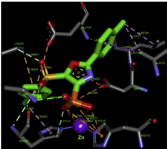
Fig. 15. Molecular docking of compound 5 into the active site of FBA-II C. albicans .
