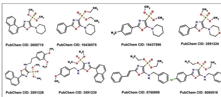
Fig. 4. Structures of FBA-II M. tuberculosis inhibitors from the PubChem bioassay AID:588726.
