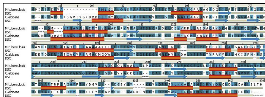
Fig. 2. A comparison of secondary structure, binding sites and active sites of FBA-II C. albicans and FBA-II M. tuberculosis by Accelrys DS.
