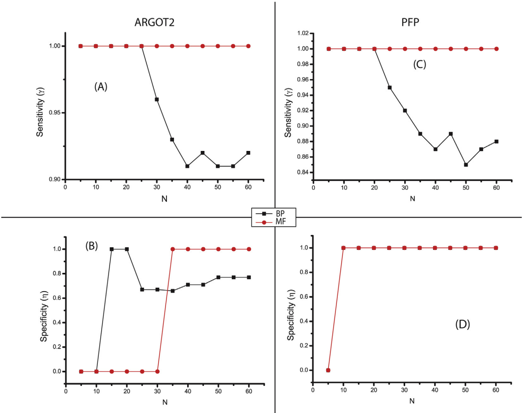
Fig. 2. ROC plots presenting the change of trend of specificity and sensitivity at different sample size (N) respectively for both Argot2 and PFP tools. Where A,B refers to Argot2 and C,D to PFP. Black lines refer to Biological process (BP) and red lines refer to Molecular function (MF).
