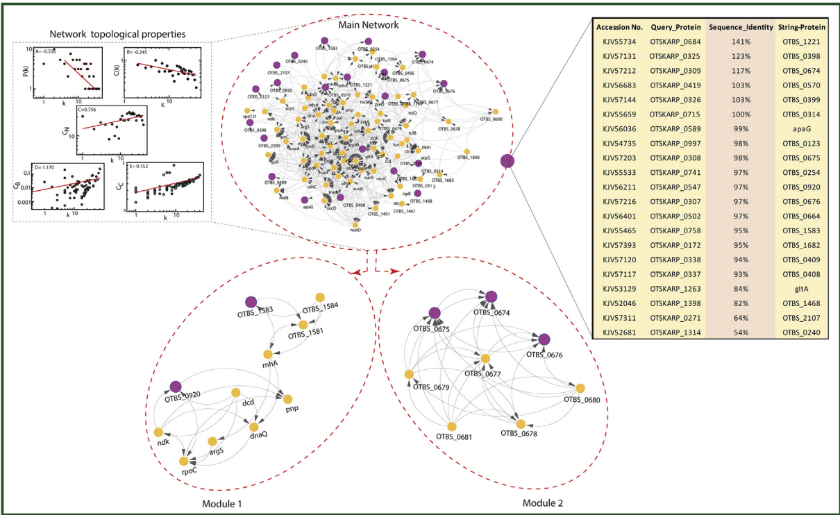
Fig. 3. Protein-Protein interaction network (cluster coeff. = 0.6) was constructed by STRING database using 62 most virulent proteins, but out of which only 21 proteins (Magenta colour nodes) interact with other proteins (yellow nodes). The topological properties show the hierarchical pattern of the network, The behaviours of degree distributions (P(k)), clustering co-efficient (C(k)), neighborhood connectivity (CN(k)), betweenness (CB(k)) and closeness (CC(k)) measurements as a function of degree k. The lines are fitted lines with power laws in the data sets. The parent network was broken into 2 highly interconnected modules (cluster coeff. = 1) which contains five hub proteins namely KJV55465(OTBS_1583),KJV56211(OTBS_0920), KJV57212(OTBS_0674), KJV57203 (OTBS_0675) and KJV57216 (OTBS_0676).
