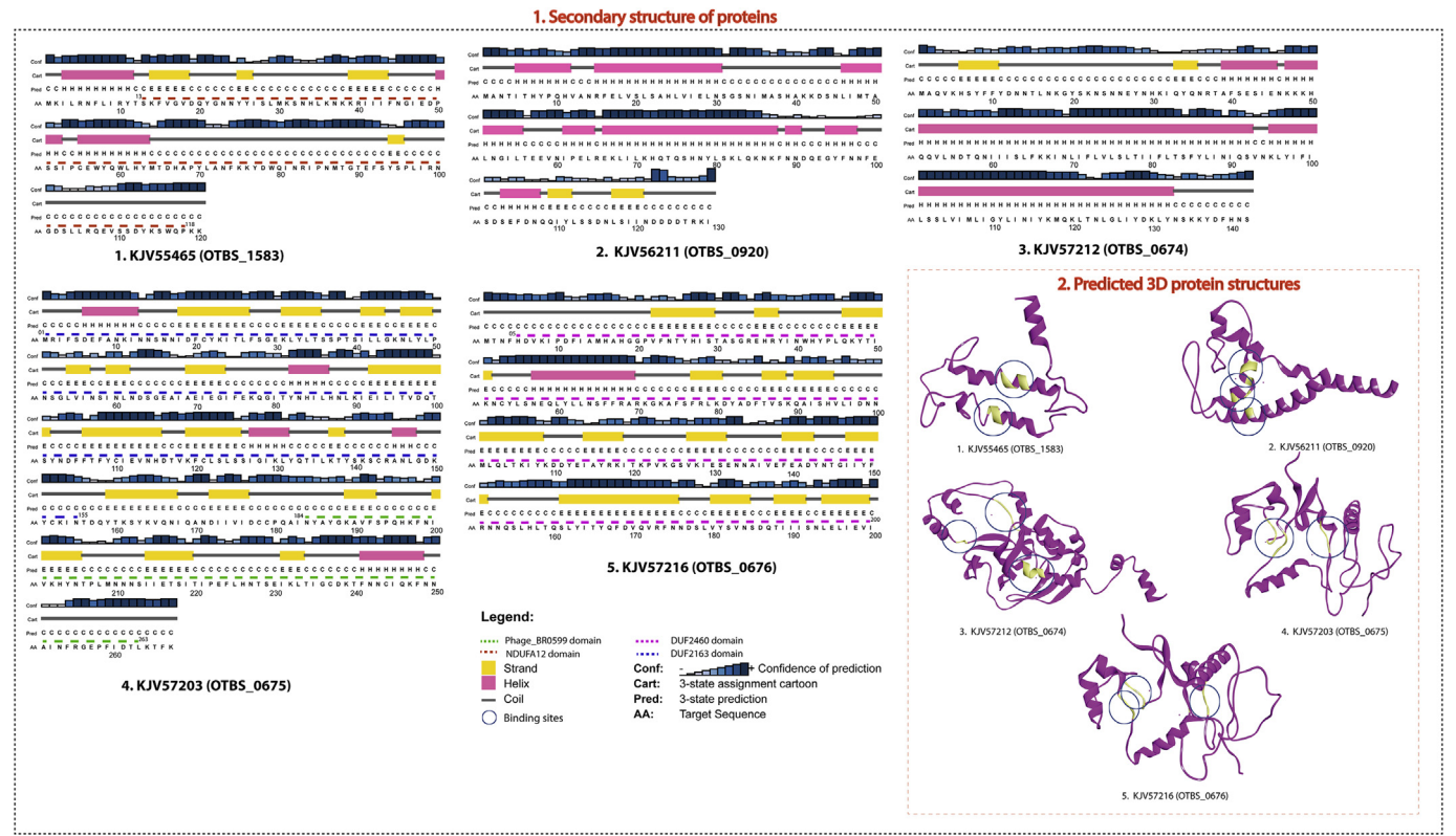
Fig. 4. Secondary structure of hub proteins predicted with the Psipred server. (1) The Psipred model showed; alpha helices, strand and coil regions and result accuracy. The confidence prediction scores are shown in the blue, grey or black bars. The red dashed line shows the conserved functional domain in the proteins. (2) The 3D structure of the five hub proteins are modelled by MODELLER and the predicted probable binding sites are circled (oily yellow) in the structures.
