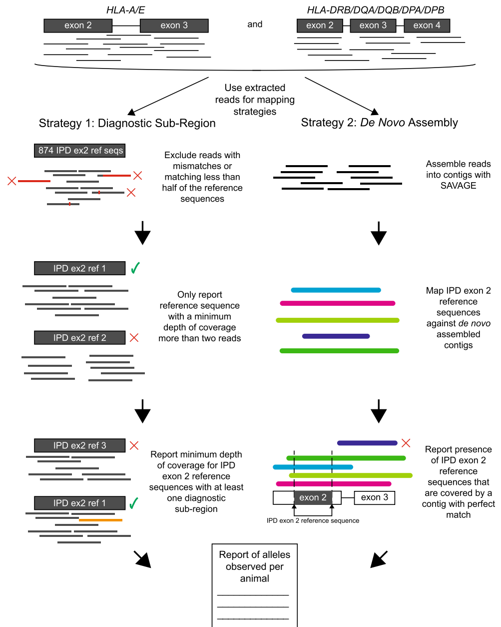
Fig. 3 Description of strategies employed for MHC genotyping from macaque exome sequencing. Exome sequencing reads are extracted by mapping to HLA-A/E exons 2–3 and HLA-DRB/DQA/DQB/DPA/DPB exons 2–4. These extracted sequences are then used for both analysis strategies. Strategy 1 maps the extracted reads to IPD exon 2 reference sequences. Only reads with perfect matches that extended off the end of contigs for no more than half of the length of the mapped read segment were retained. Next, each alignment of mapped sequences is checked to exclude those with a coverage that is less than 2 reads. The mapped alignments with this coverage are used to form a diagnostic subread, which is used to match alignments to the reference sequences. The minimum depth of coverage of the mapped alignments was reported in the output. Strategy 2 conducts a de novo assembly of the extracted reads using the computational tool SAVAGE. Then, the assembled contigs are mapped to IPD exon 2 reference sequences. To determine correct mapping, any IPD exon 2 reference sequences that fully cover and perfectly match a contig are reported in the output
