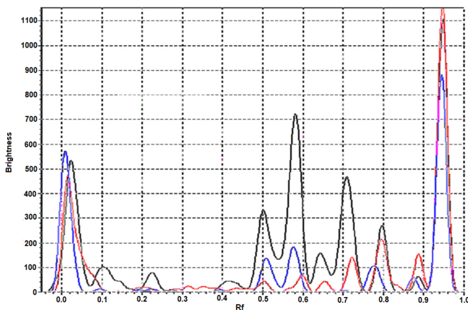
Fig. 4. Densitogram of Astragalus danicus L. samples (365 nm): black line – Prokopyevsky district, red line – Yashkinsky district, blue line – Belovsky district.
