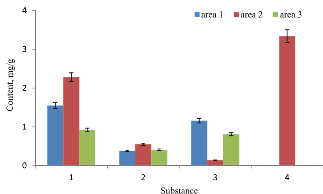
Fig. 5. The content of phenolic compounds of Astragalus danicus L. samples from Prokopyevsky district (area 1), Yashkinsky district (area 2), Belovsky district (area 3): 1 - isorhamnetin glucoside; 2 - kaempferol glucoside; 3 - apigenin 7-glucoside; 4 - chlorogenic acid.
