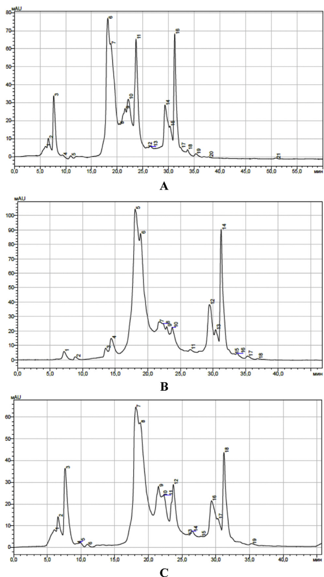
Fig. 3. Chromatogram of Astragalus danicus alcohol extract sample: A collection area 1; B collection area 2; C collection area 3.
