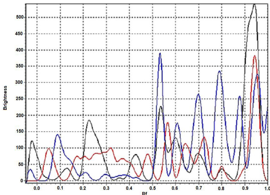
Fig. 2. Densitogram of Astragalus danicus samples after developing by diazoreactive: black line – Prokopyevsky district, red line – Yashkinsky district, blue line – Belovsky district.
