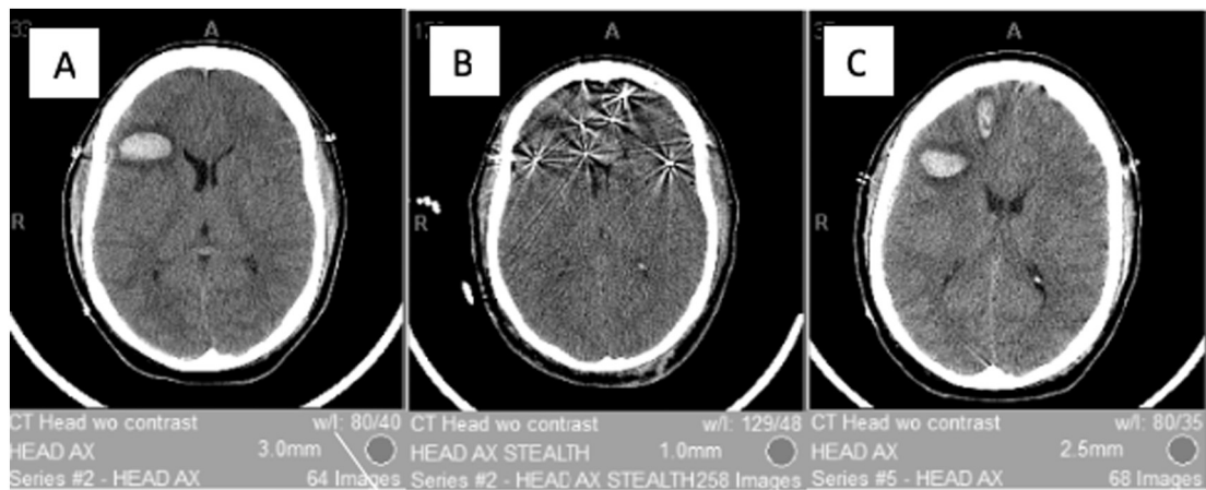
Fig. 4. A. Postexplantation CT with new onset of right posterior orbitofrontal hemorrhage. B. Postimplantation CT without hemorrhage. C. Evolution of right POF hemorrhage and subsequent new onset frontal hemorrhage at 2 days post discharge.
