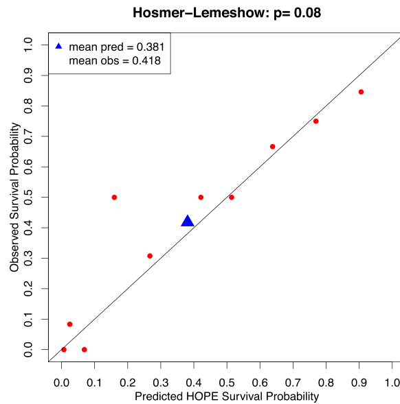
Fig. 3 – Observed probability of survival according to the predicted survival rate in the validation sample ( n = 122 ). Each one of the red plots represent a decile of the predicted survival probabilities in the whole derivation sample. The Hosmer–Lemeshow ( p = 0.08 ) indicates that the differences between observed and predicted survival probabilities are not significant, indicating good calibration of the model (for interpretation of the references to colour in this figure legend, the reader is referred to the web version of this article).
