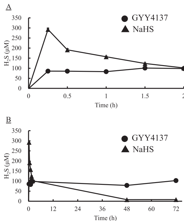
Fig. 1. Release of \text{H}_2\text{S} by GYY4137 (1.0 mM, ●) and NaHS (1.0 mM, ▲) into culture medium. (A) \text{H}_2\text{S} release was determined at time intervals up to 2 h. (B) \text{H}_2\text{S} release was determined at time intervals up to 72 h. Data are expressed as the mean \pm SEM ( n = 4 ).
