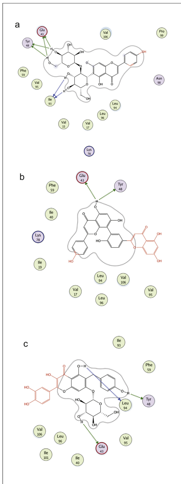
Fig. 8. 2D interaction diagram, showing the interacting flavonoid atoms with specific residues in active site of BCL1 protein. Dotted lines are showing specific interaction. a) 3',4',5-trihydroxy-3-methoxyflavon-7-olate, b) Agathisflavone, c) catiguanin B.
