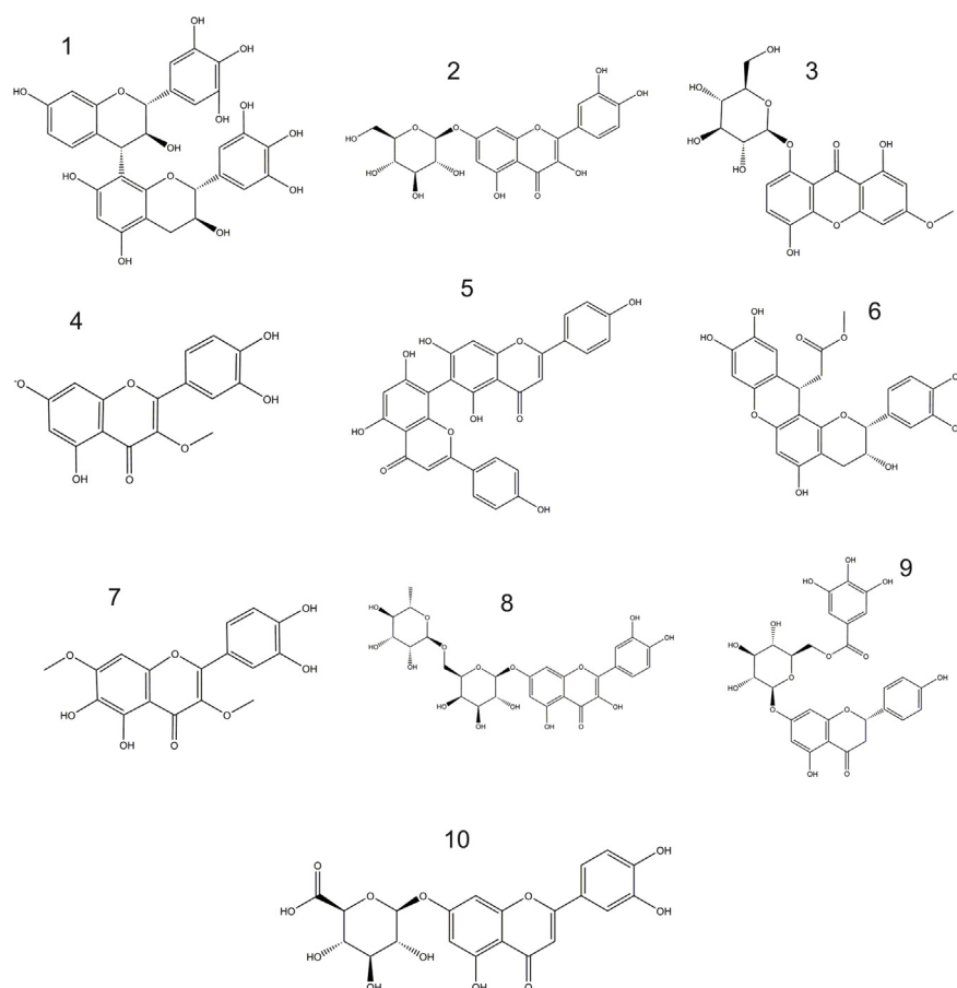
Fig. 5. Flavonoid structures showing best results of docking analysis; a) robinetinidol-(4 \alpha ,8)-gallo-catechin, b) quercetin 7-O-beta-D-glucoside, c) Swertianolin, d) 3',4',5-trihydroxy-3-methoxyflavon-7-olate, e) Agathisflavone, f) catiguanin B, g) 3',4',5,6-tetrahydroxy-3,7-dimethoxyflavone, h). quercetin-7-O-[ \alpha -L-rhamnopyranosyl(1->6)- \beta -D-galactopyranoside], i) prunin 6''-O-gallate, j) luteolin 7-O-beta-D-glucosiduronic acid.
