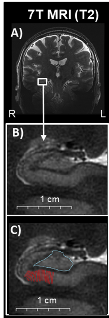
Fig. 1. Hippocampal subfields illustrations on images obtained at 7T MRI. A) Oblique coronal view of a 7T T2-weighted MRI scan. B) Magnified area of the hippocampus where subfields are readily visualized and thus able to be manually traced. C) Superimposed manual tracing of the CA1 (red) and DG/CA3 (turquoise). Abbreviations: R: right, L: left.
